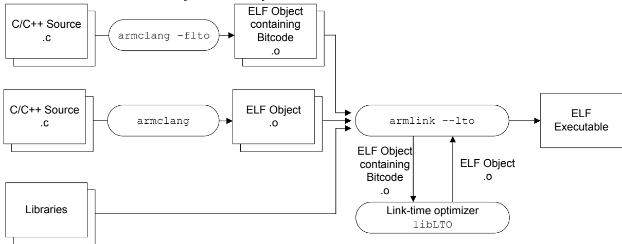
Figure 3-7 Link-Time Optimization
