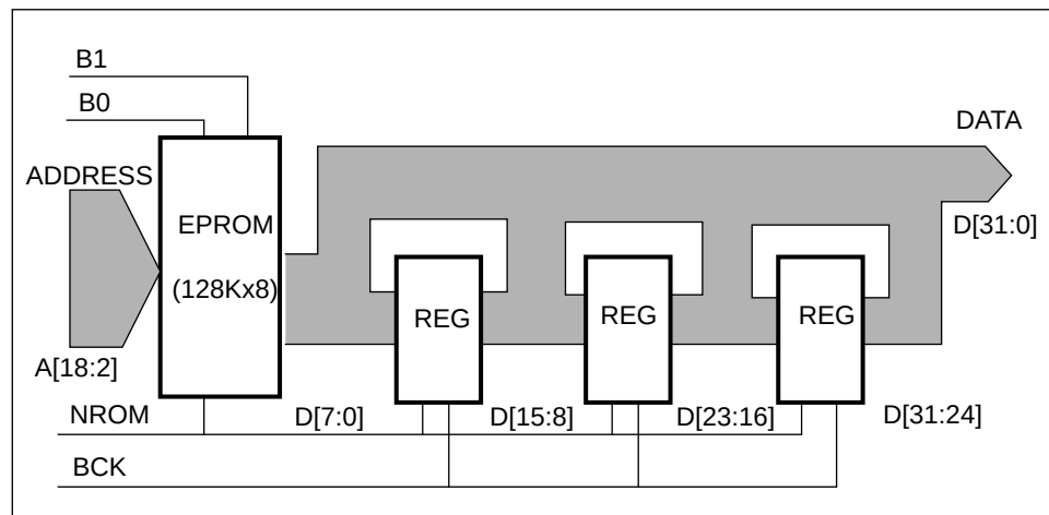
Figure 3.6 EPROM pipeline
