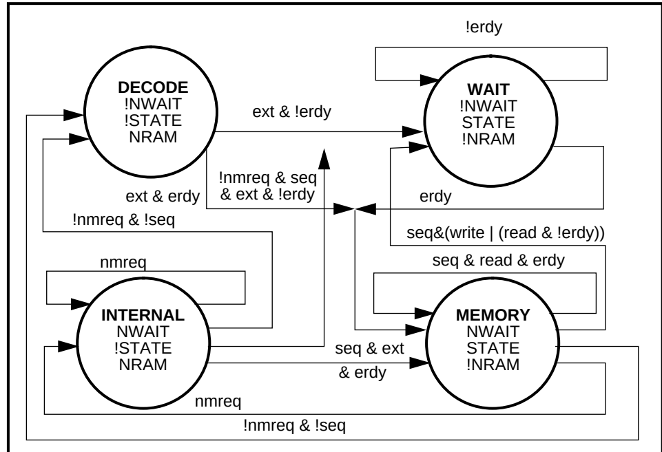
Figure 5.11 External I/O access state diagram
