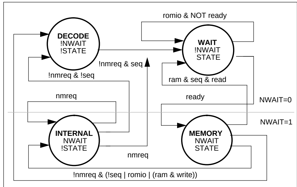
Figure 5.6 Expanded state diagram
