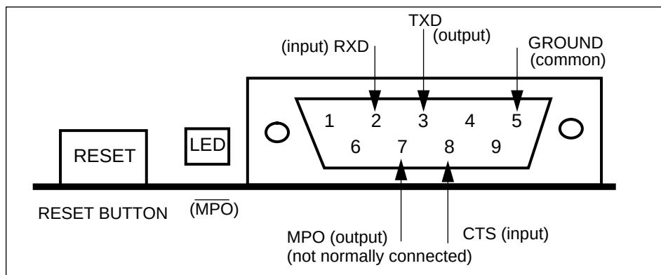
Figure A.1 Connector (View from end of card)
