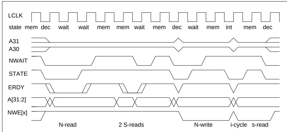
Figure 5.10 SRAM Waveforms
