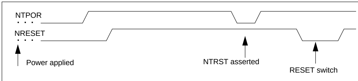
Figure 3.10 Reset timing
