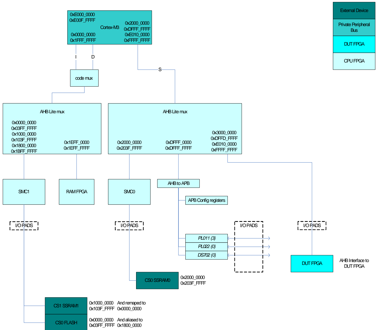
Figure 4: CPU FPGA Bus Architecture
