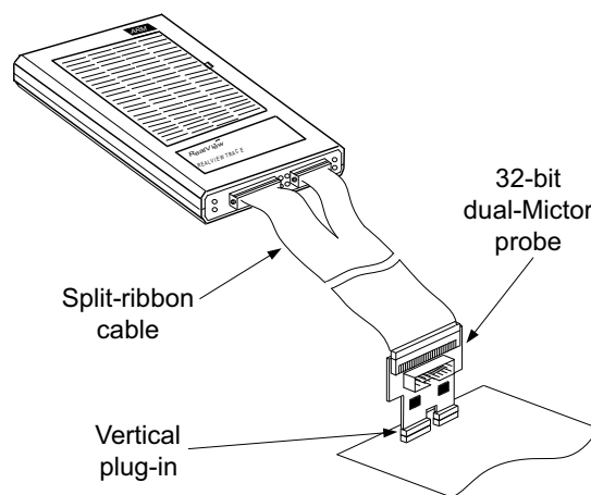
Figure 6-4 RVT2 unit connections
