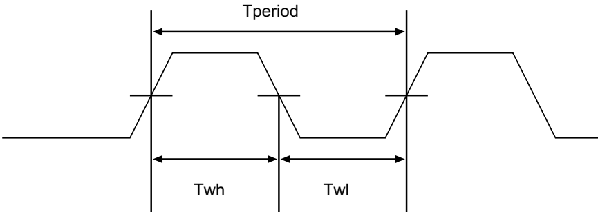
Figure 5-1 Clock waveforms
