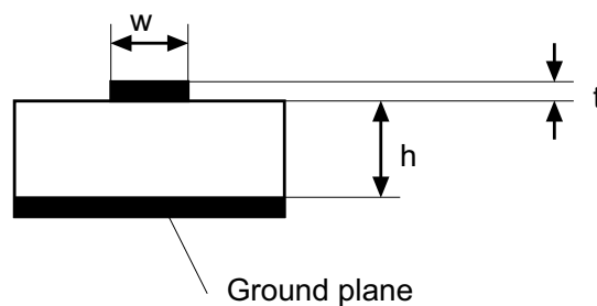
Figure 6-1 Track impedance
