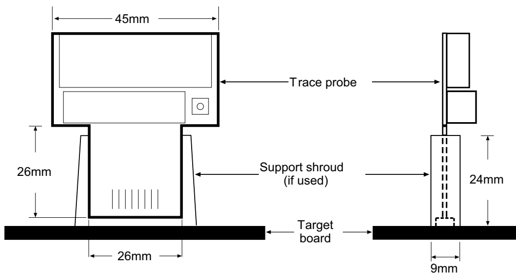
Figure 6-2 Probe dimensions
