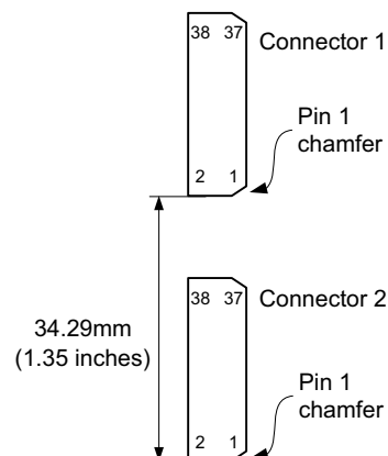
Figure 6-6 Dual-Mictor pitch dimensions
