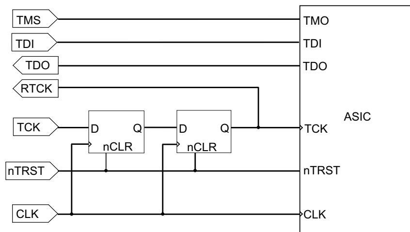
Figure 2-1 Basic JTAG port synchronizer
