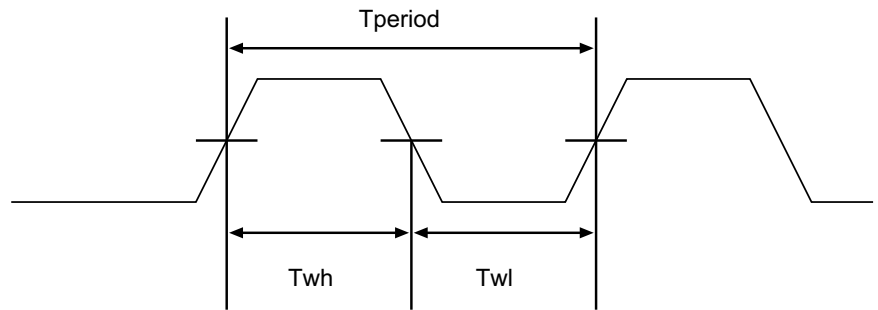
Figure 3-4 Clock waveforms
