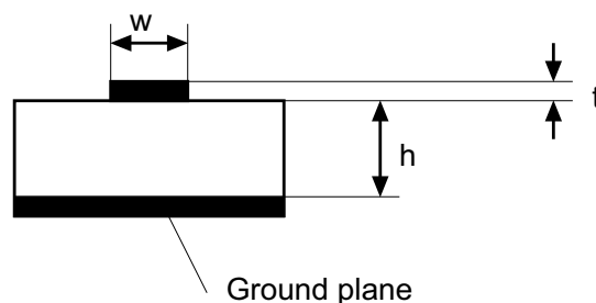
Figure 5-1 Track impedance
