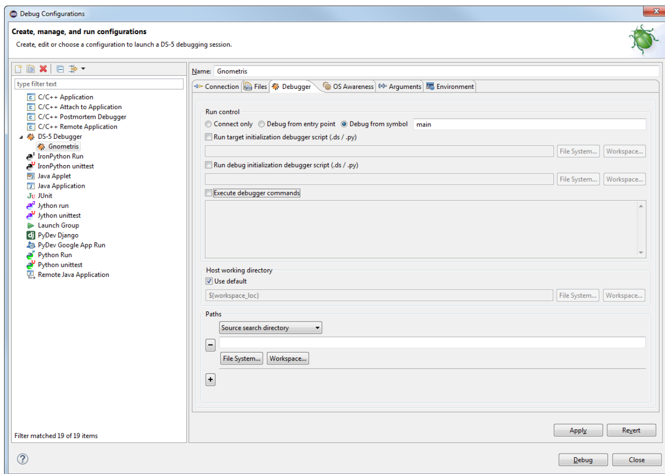
Figure 4-12 Typical debugger settings for Linux application debug
