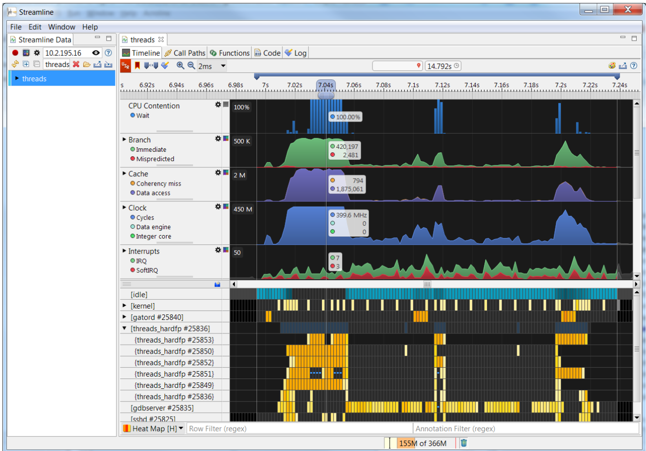
Figure 4-16 Streamline analysis report for the threads application
