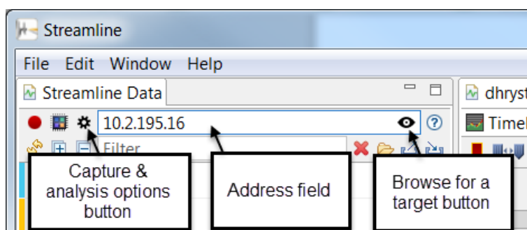
Figure 4-15 Streamline Data view
