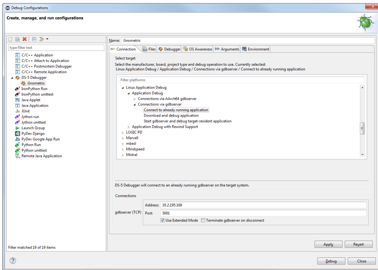
Figure 4-10 Typical connection configuration for Linux application debug
