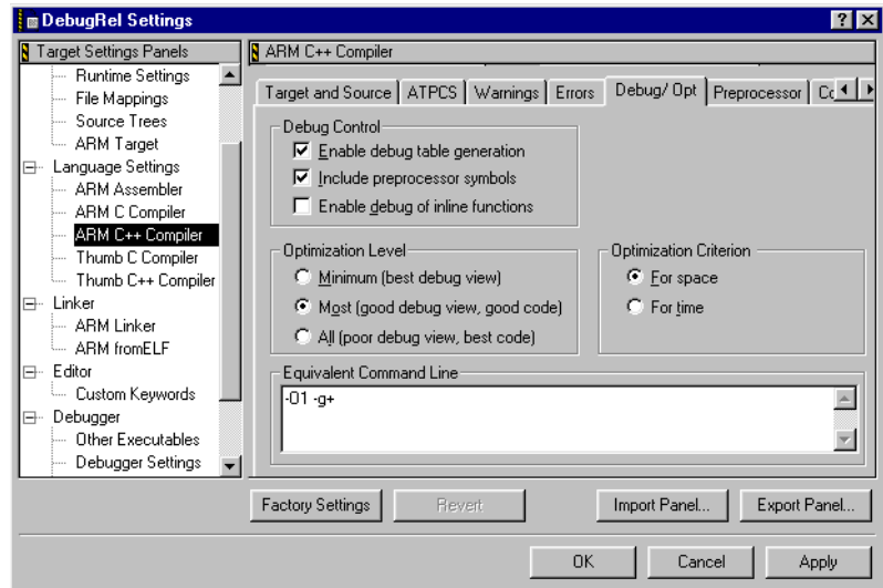
Figure 4-2 ARM compiler Debug/Opt panel
