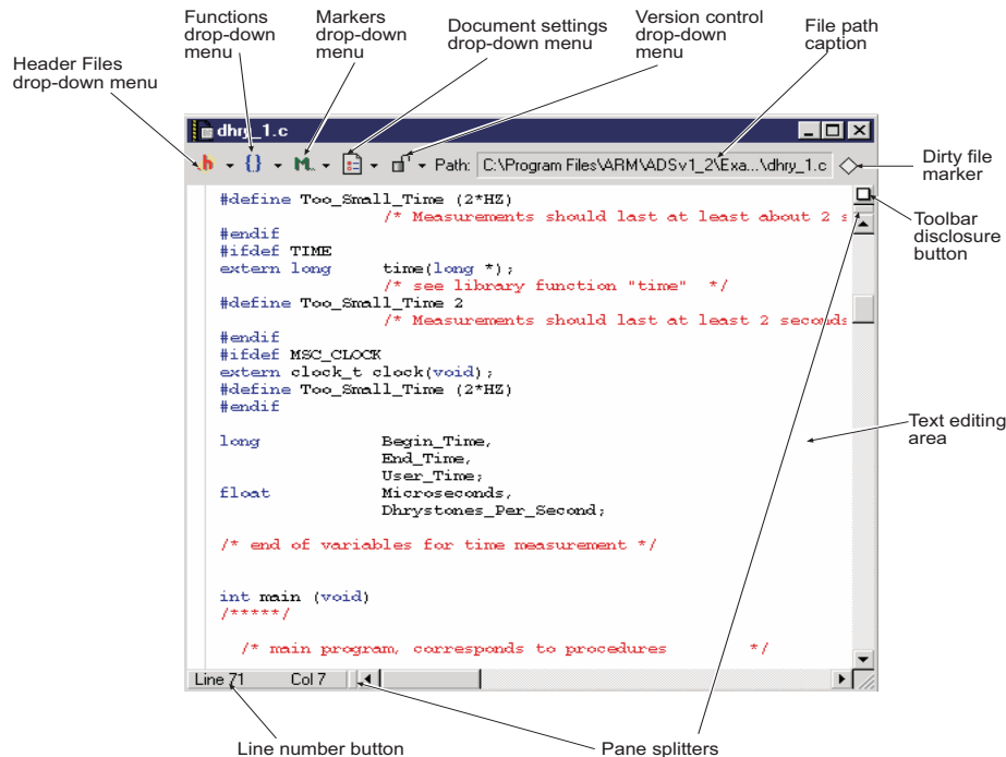
Figure 5-1 The editor window
