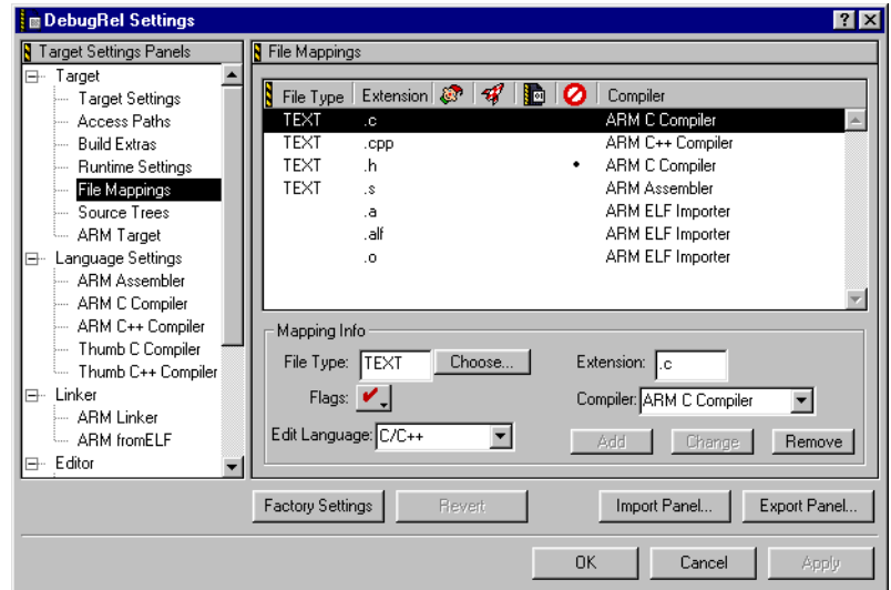
Figure C-1 File mappings configuration panel
