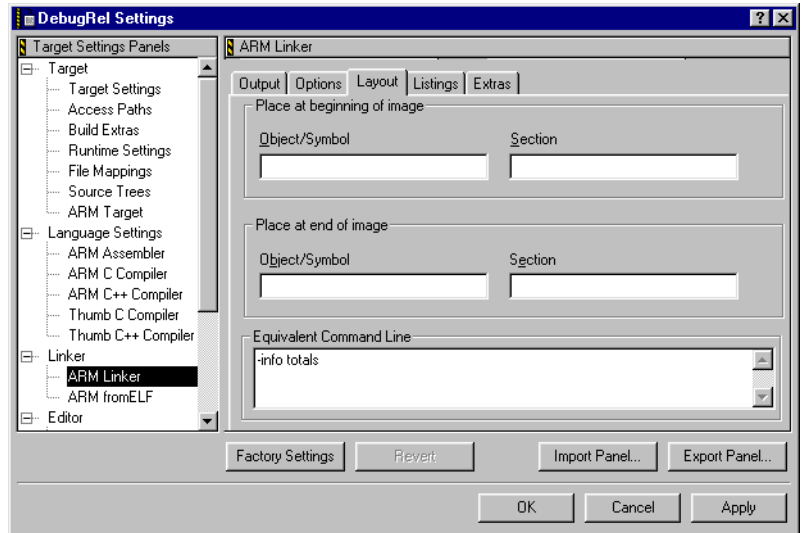
Figure 9-30 ARM Linker Layout panel
