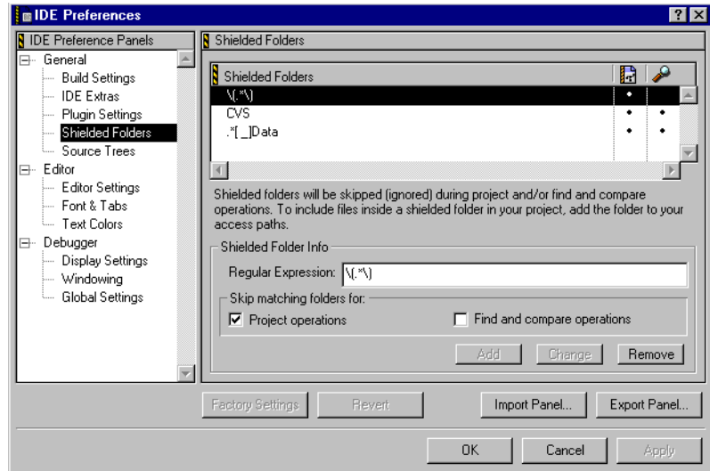
Figure 8-6 Shielded Folders settings panel
