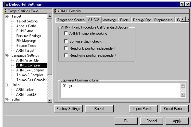
Figure 9-21 ARM compiler APCS panel
