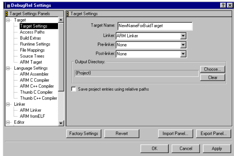
Figure 3-38 Renaming a build target
