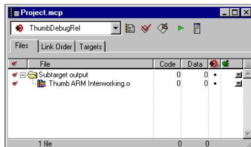
Figure 3-10 Interworking project
