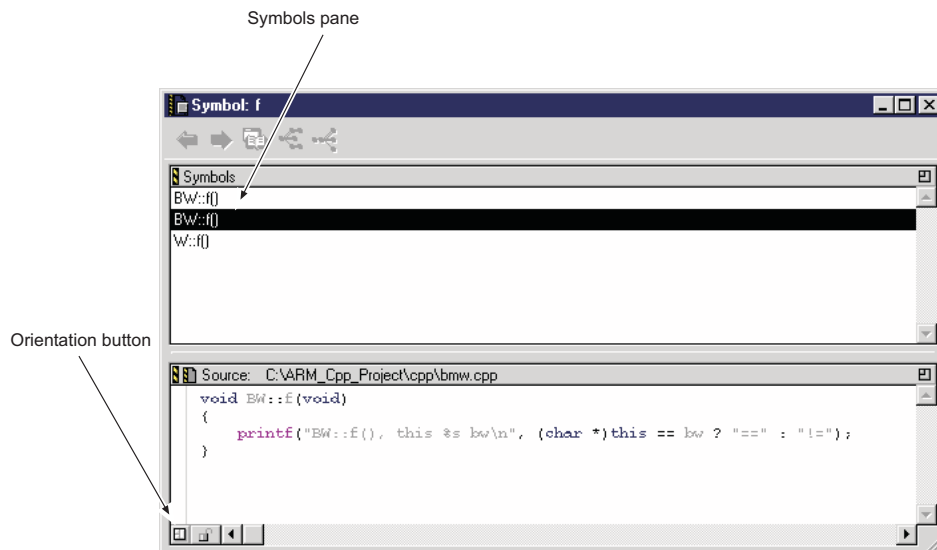
Figure 7-15 The Symbol window
