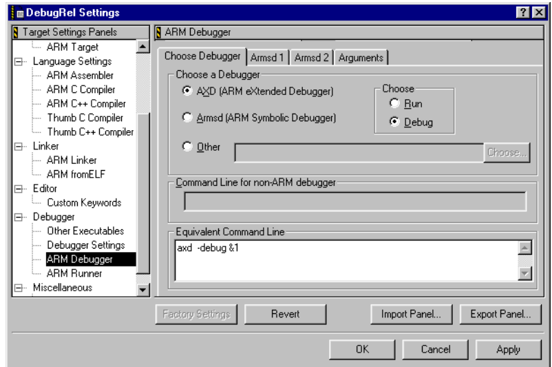
Figure 9-35 Choose debugger panel
