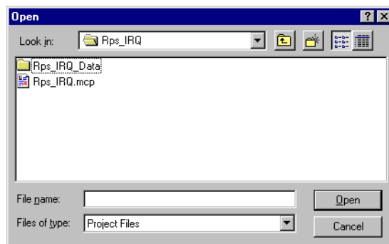
Figure 3-7 Open dialog
