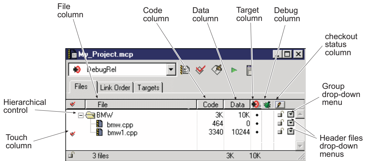
Figure 3-2 Project window Files view
