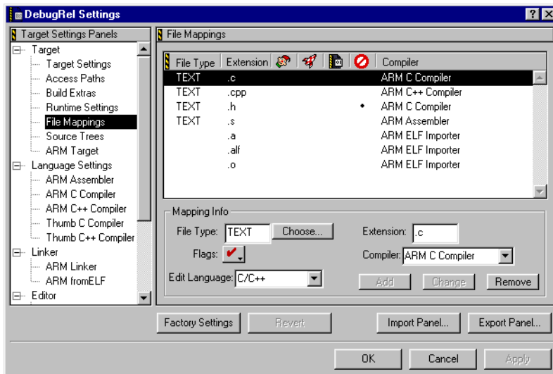
Figure 3-56 File Mappings panel
