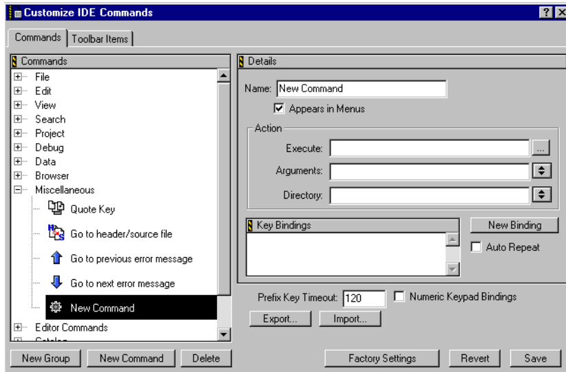
Figure 8-14 Configuring a new command
