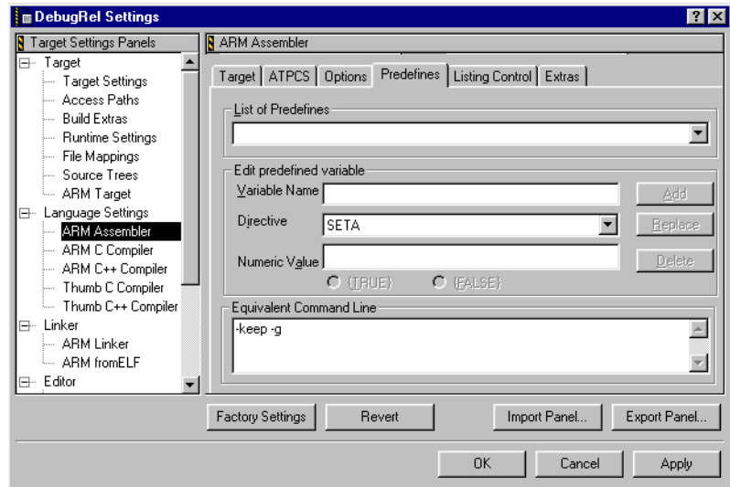
Figure 9-17 ARM Assembler Predefines panel
