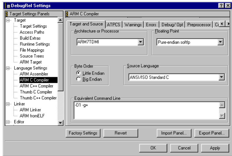
Figure 9-20 ARM compiler Target and Source panel
