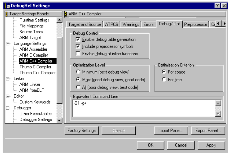
Figure 9-24 ARM compiler Debug and optimization panel
