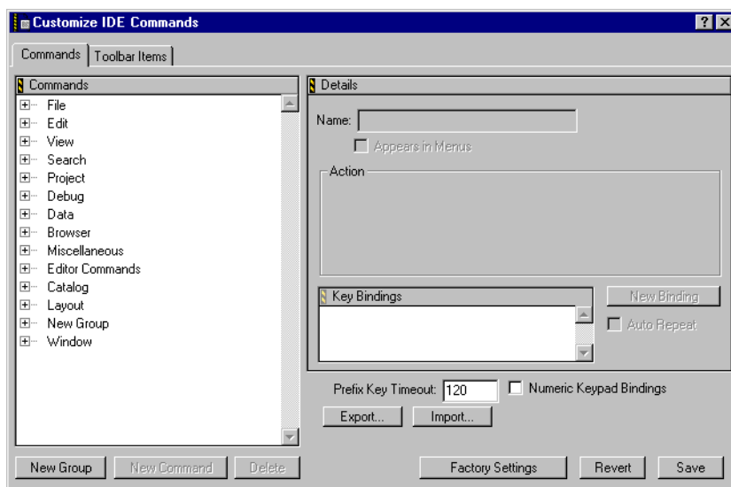
Figure 8-22 Customize IDE Commands window
