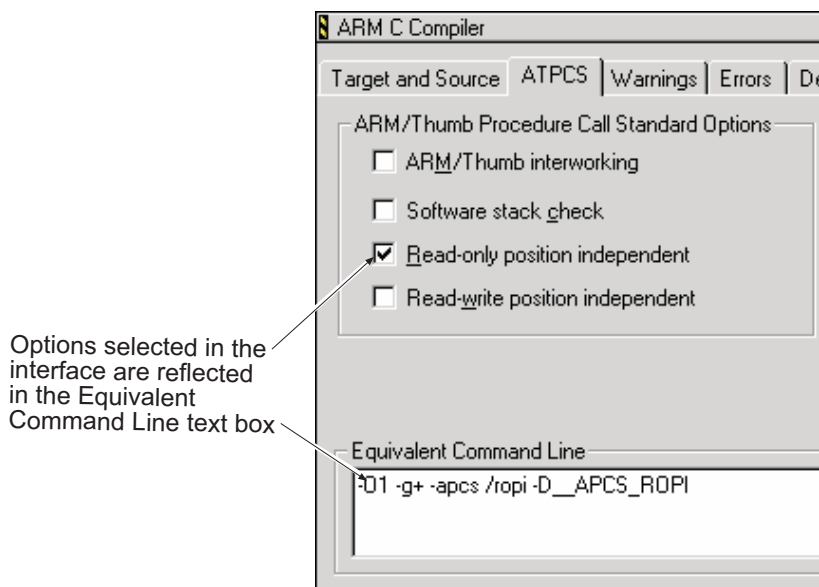
Figure 9-13 Equivalent Command Line text box
