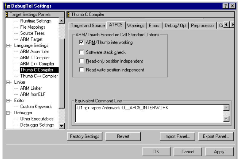
Figure 3-19 Selecting the ATPCS Interworking option
