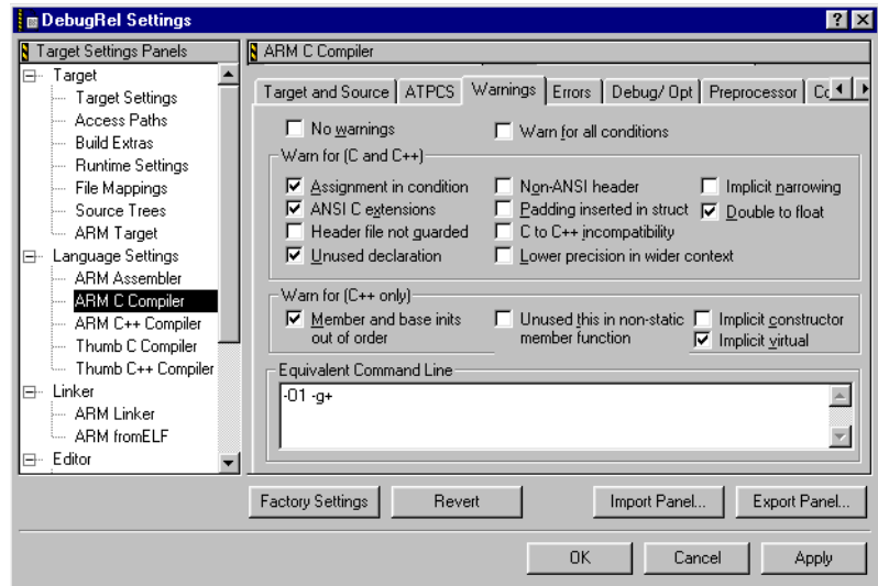
Figure 9-22 ARM compiler Warnings panel
