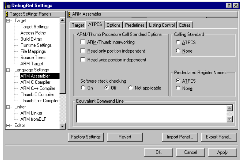
Figure 9-15 ARM Assembler ATPCS panel
