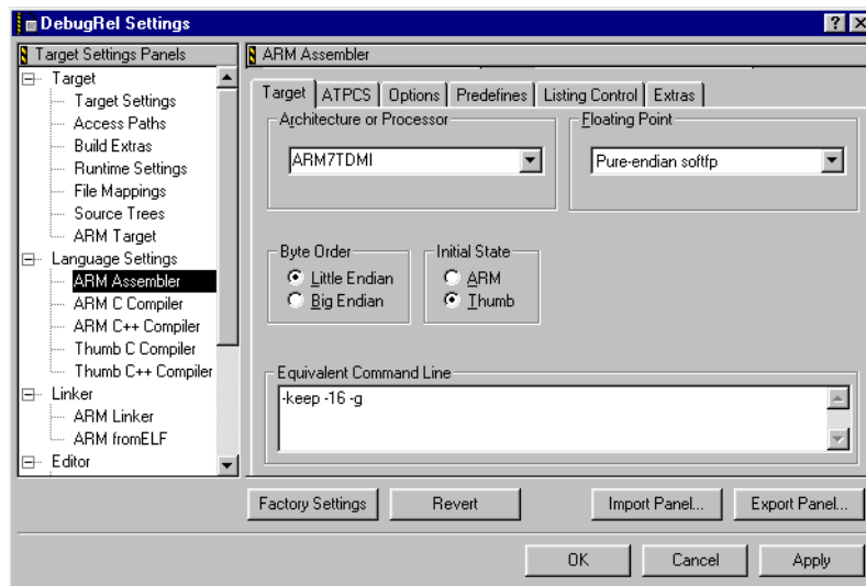
Figure 3-17 Select Thumb initial state
