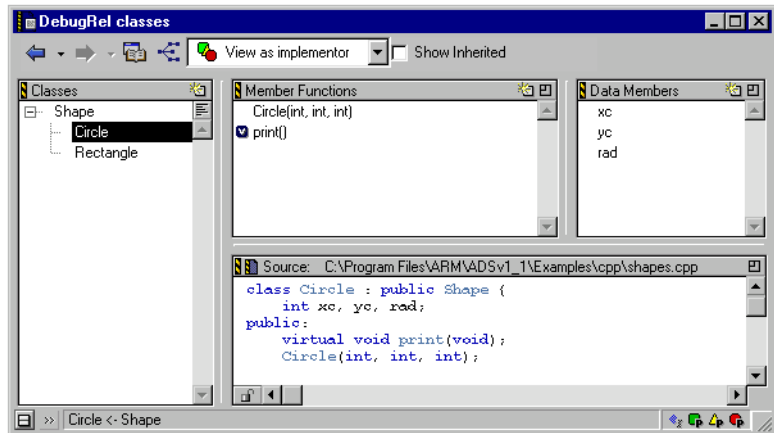
Figure 7-4 Member functions, data members, and declaration for class circle
