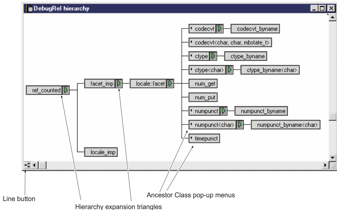
Figure 7-8 The Multi-class hierarchy window
