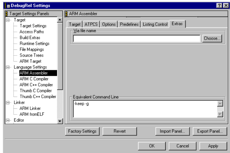
Figure 9-19 ARM Assembler Extras panel
