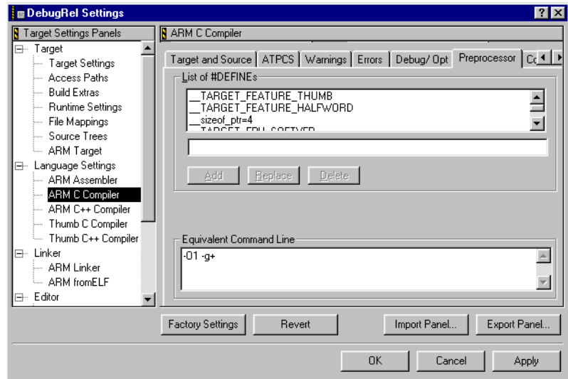
Figure 9-25 ARM compiler Preprocessor panel
