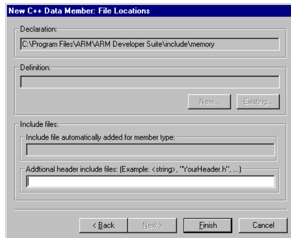
Figure 7-25 New Data Member wizard: File Locations
