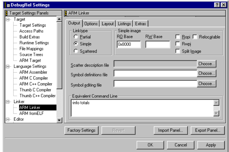
Figure 9-28 ARM linker Output panel
