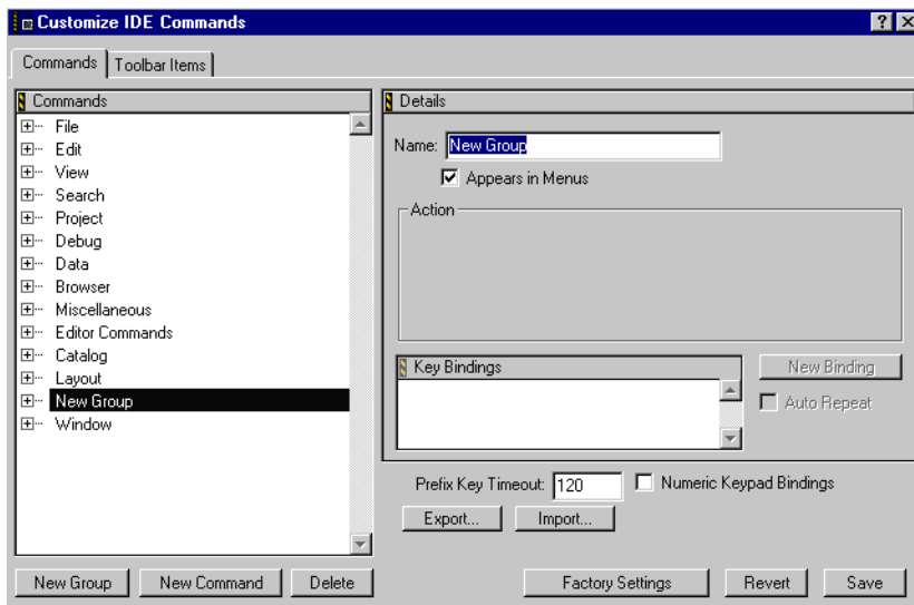
Figure 8-16 Creating a new group
