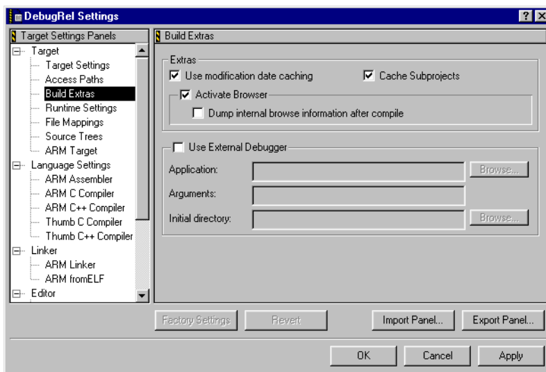
Figure 7-1 Target settings panel
