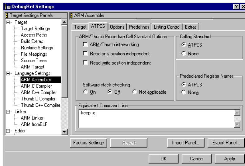
Figure 3-18 Select ARM/Thumb interworking
