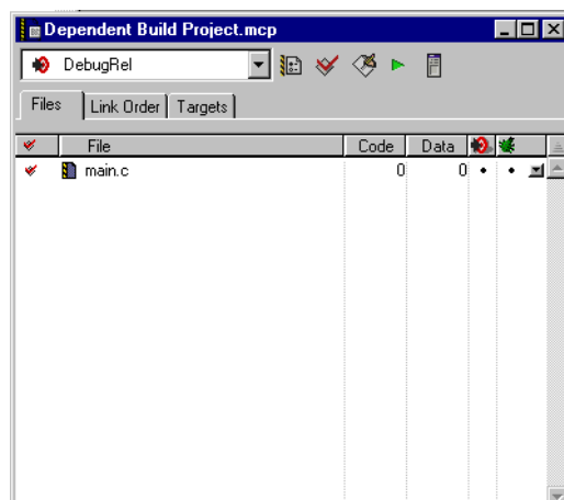
Figure 3-39 Project window
