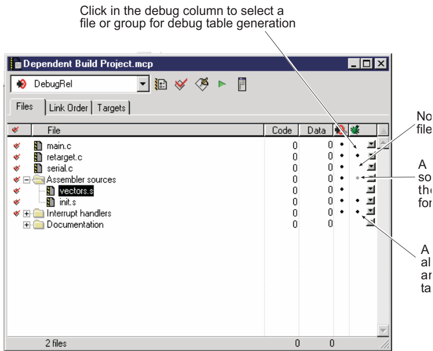
Figure 4-1 Debug Info markers
