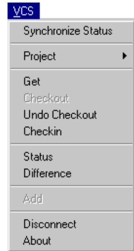
Figure 10-4 VCS menu
