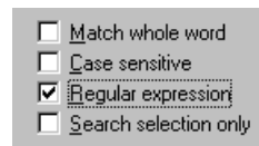
Figure 6-10 Regexp checkbox
