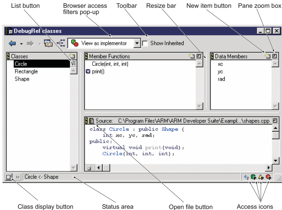
Figure 7-2 A Class browser view
