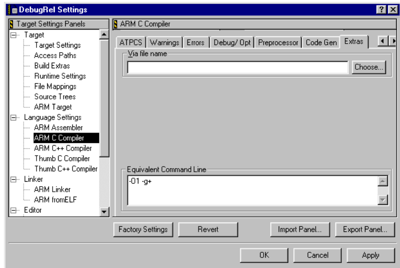
Figure 9-27 ARM Compiler Extras panel
