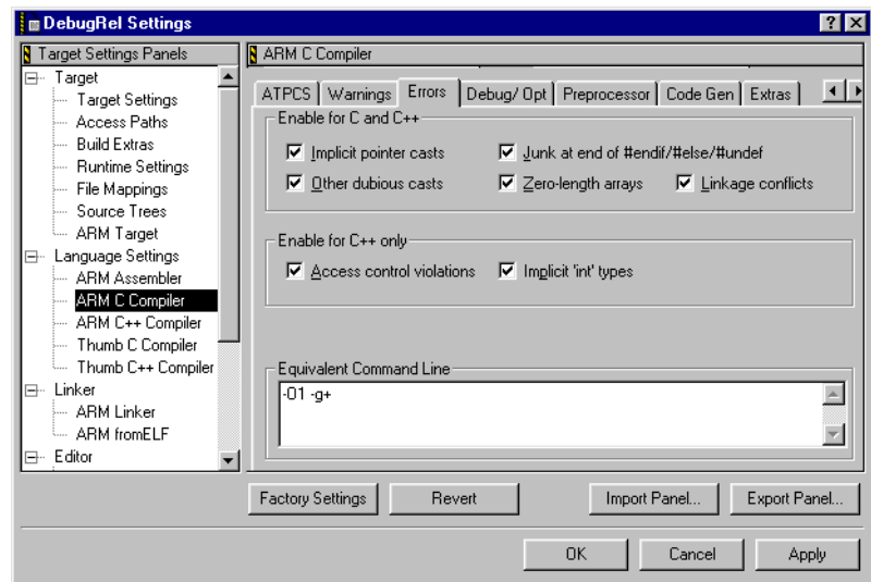
Figure 9-23 ARM compiler Errors panel
