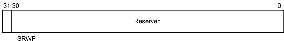
Figure 3-8 GICD_ESTATUSR bit assignments
