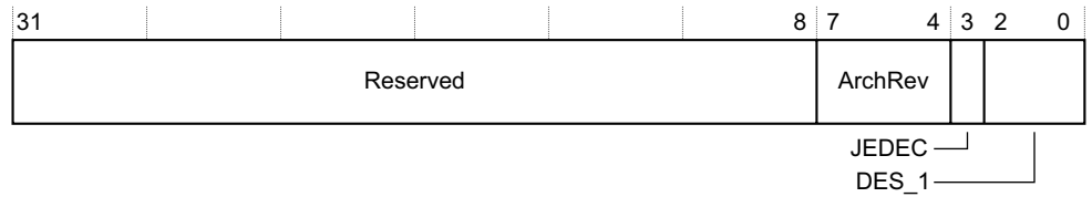
Figure 3-2 GICD_PIDR2 bit assignments
