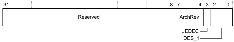
Figure 3-7 GITS_PIDR2 bit assignments
