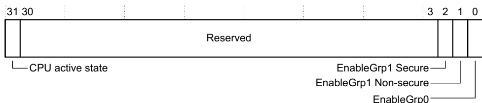
Figure 3-11 GICR_MISCSTATUSR bit assignments
