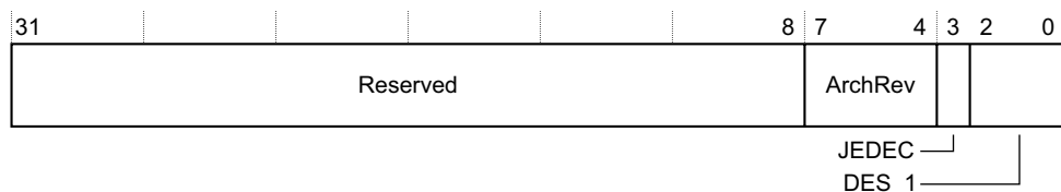
Figure 3-5 GICR_PIDR2 bit assignments
