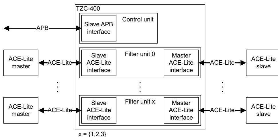
Figure 1-1 TZC-400 overview
