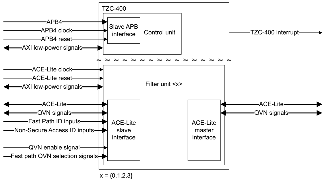
Figure 2-1 TZC-400 interfaces
