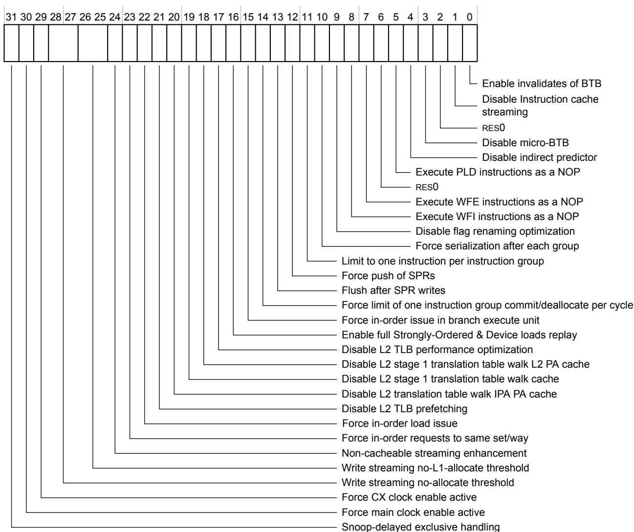
Figure 4-74 CPUACTLR_EL1[31:0] bit assignments
