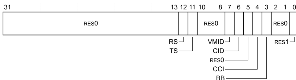
Figure 13-2 TRCCONFIGR bit assignments
