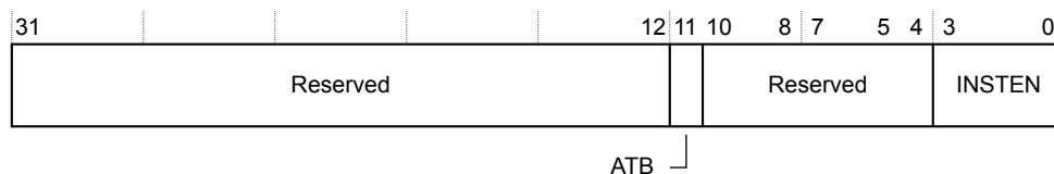
Figure 13-5 TRCEVENTCL1R bit assignments
