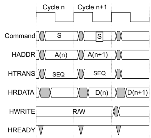
Figure 7-7 Sequential command timing
