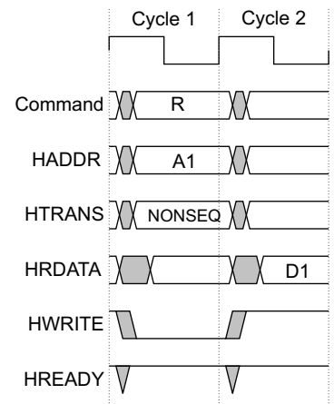
Figure 7-6 Read command timing
