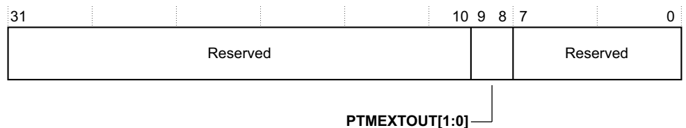
Figure 12-12 ITMISCOUT bit assignments
