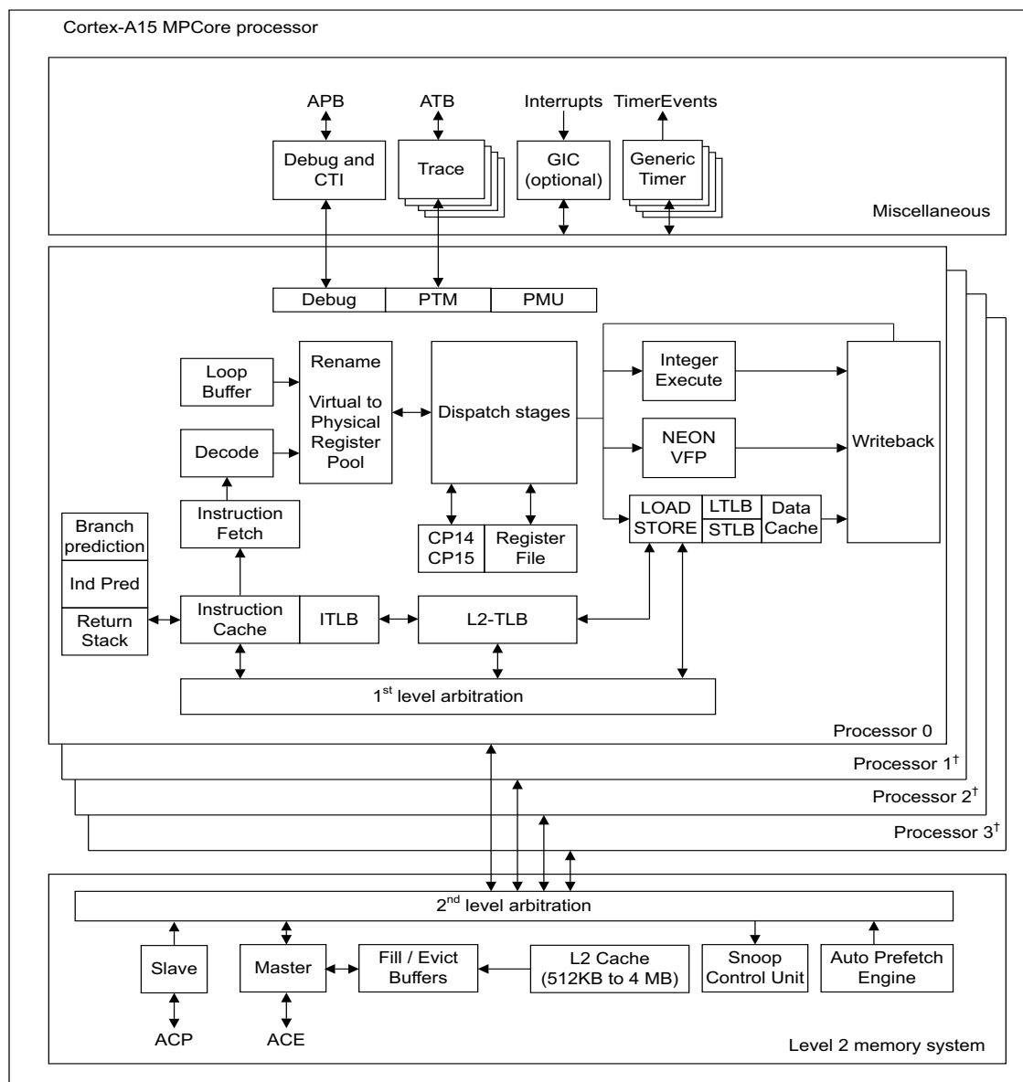
Figure 2-1 Block diagram
