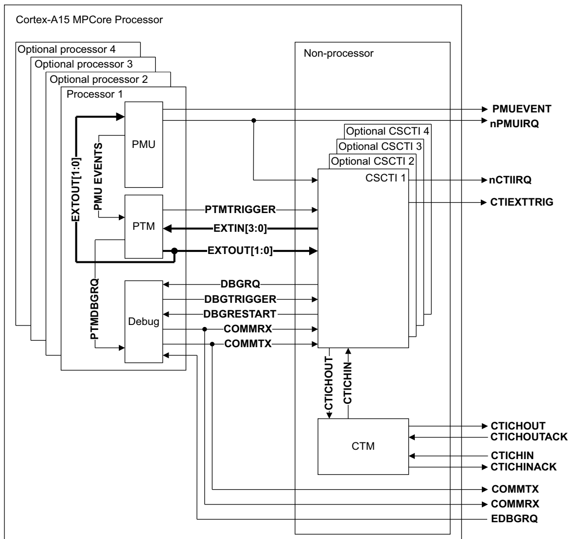
Figure 13-1 Debug system components
