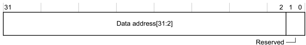
Figure 10-8 DBGWVR bit assignments
