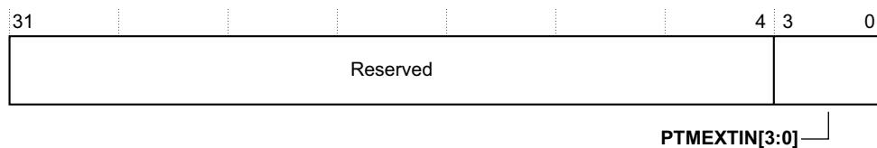
Figure 12-13 ITMISCIN bit assignments
