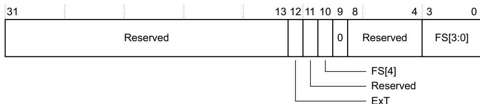
Figure 4-33 IFSR bit assignments for Short-descriptor translation table format
