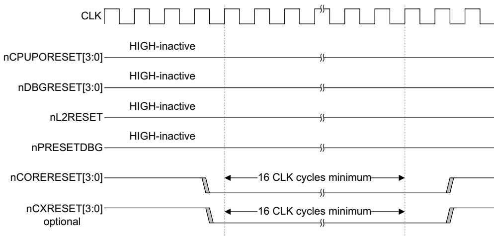
Figure 2-8 Soft reset timing
