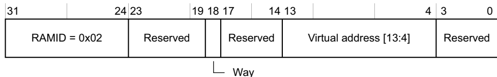
Figure 4-45 RAMINDEX bit assignments for L1-I BTB RAM
