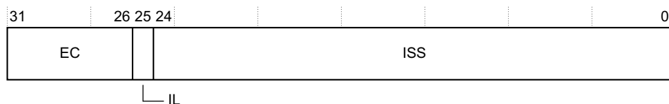
Figure 4-37 HSR bit assignments
