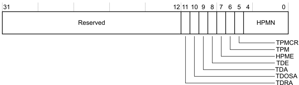
Figure 4-29 HDCR bit assignments
