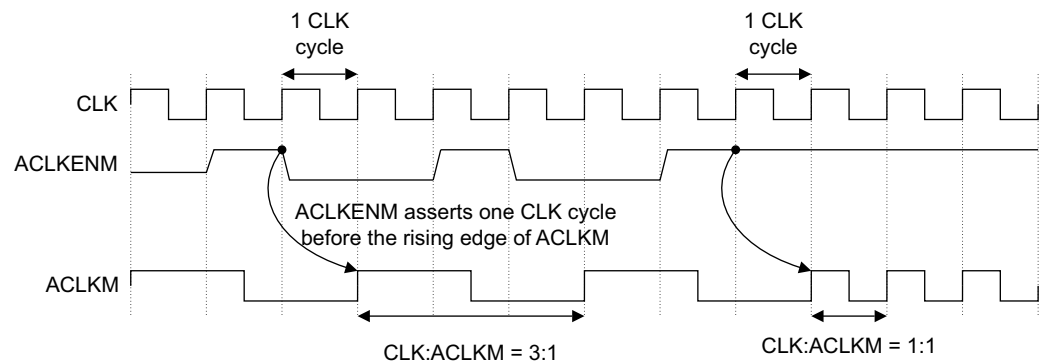
Figure 2-2 ACLKENM with CLK:ACLKM ratio changing from 3:1 to 1:1
