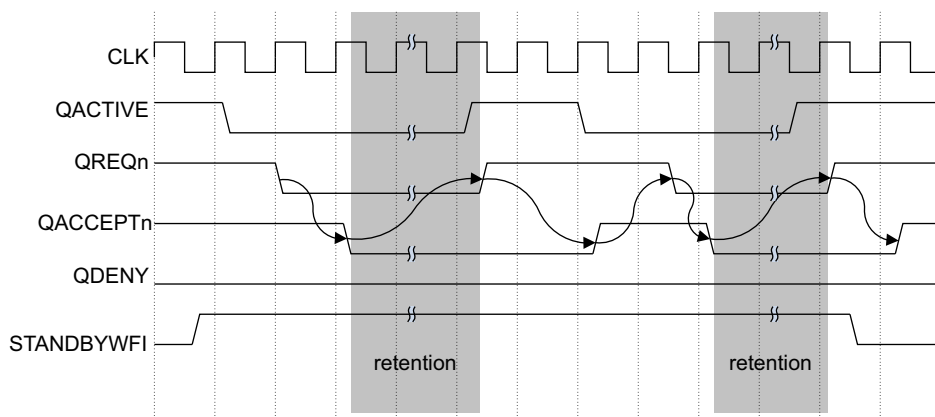
Figure 2-14 WFI successful retention timing
