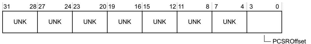
Figure 10-23 DBGDEVID1 bit assignments
