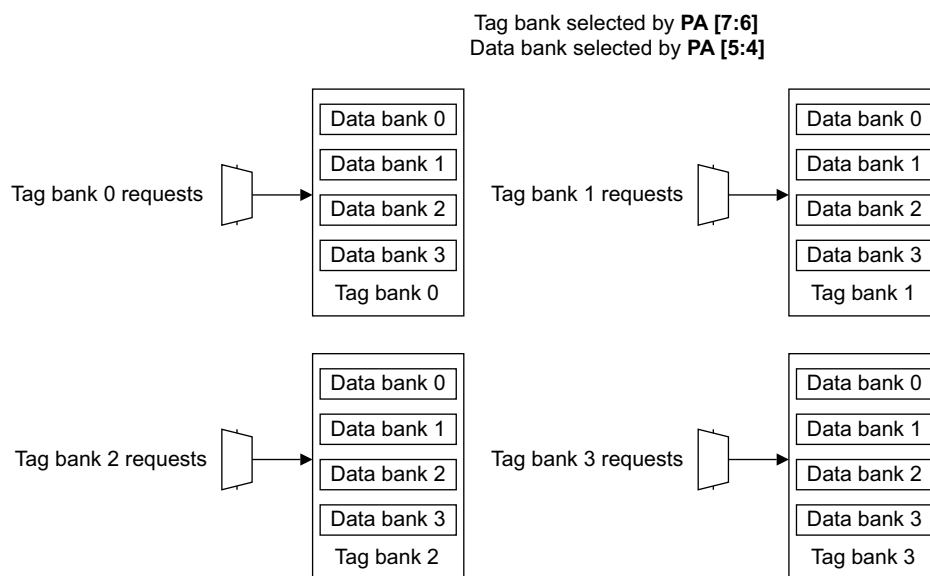
Figure 7-1 L2 cache bank structure
