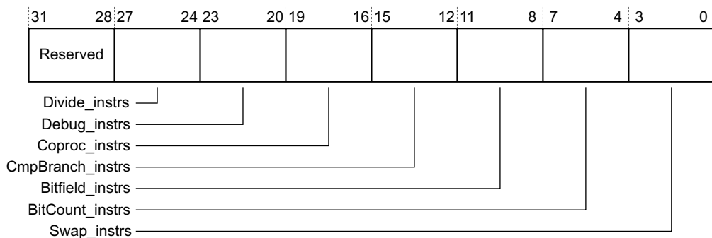
Figure 4-13 ID_ISAR0 bit assignments
