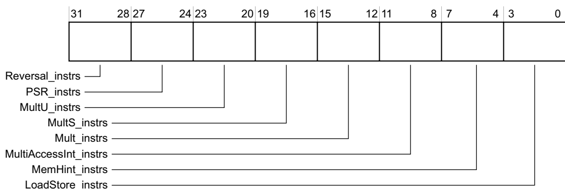
Figure 4-15 ID_ISAR2 bit assignments
