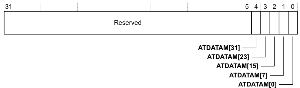
Figure 12-15 ITATBDATA0 bit assignments
