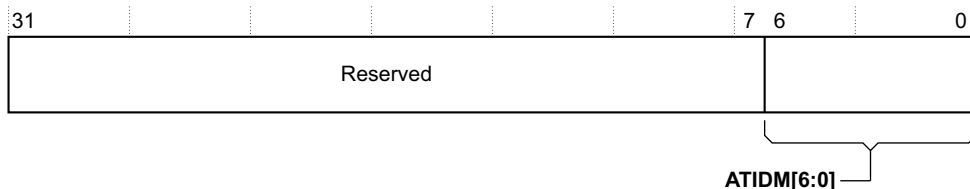
Figure 12-17 ITATBID bit assignments
