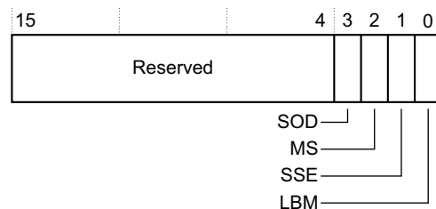
Figure 3-2 SSPCR1 Register bit assignments
