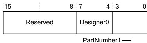
Figure 3-13 SSPPeriphID1 Register bit assignments
