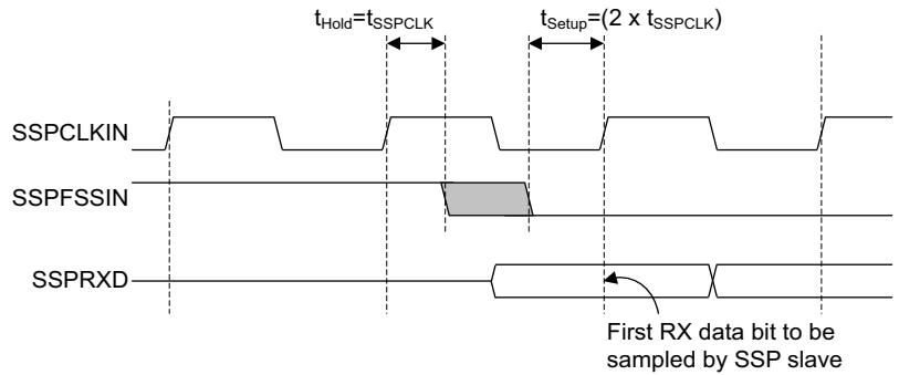
Figure 2-12 Microwire frame format, SSPFSSIN input setup and hold requirements
