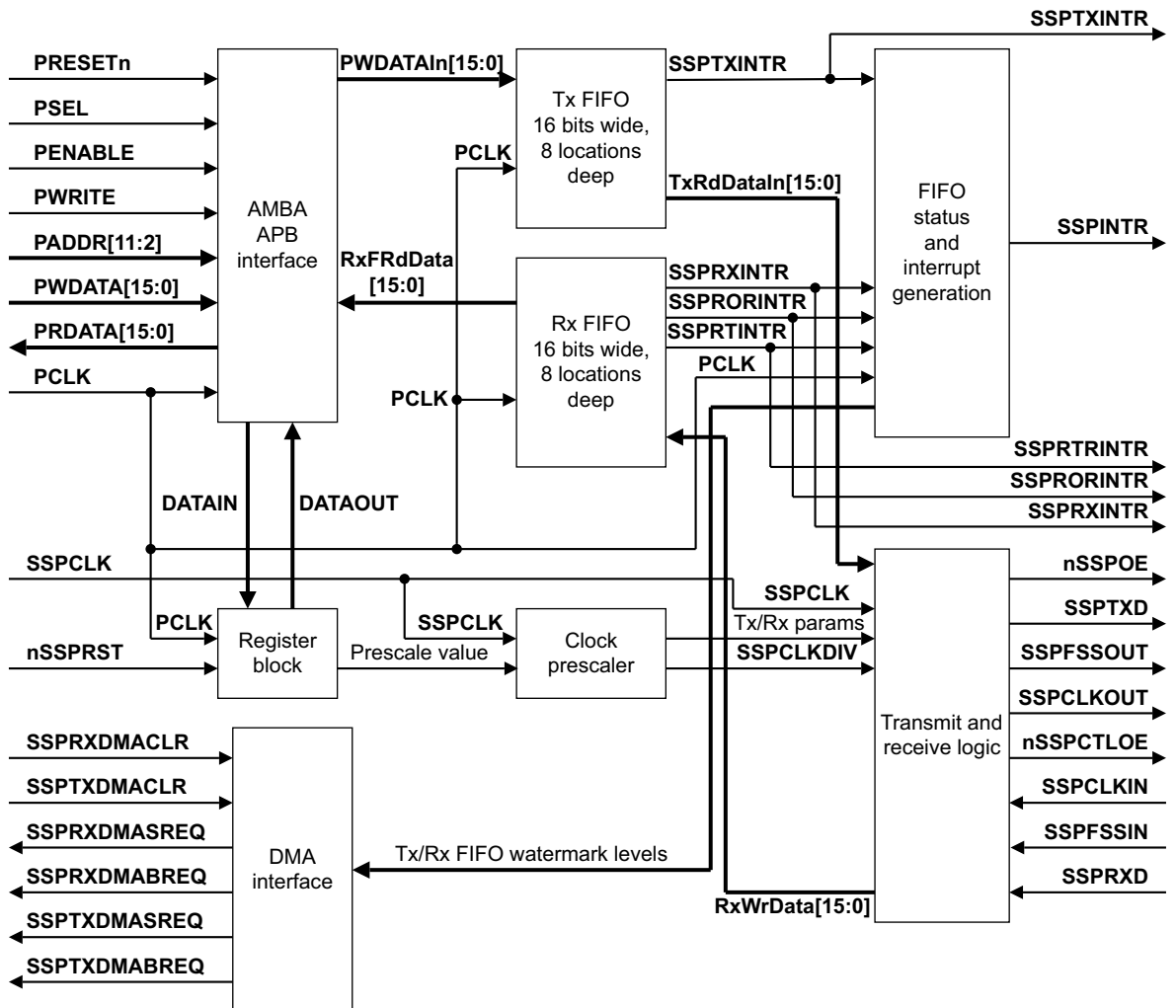
Figure 2-1 PrimeCell SSP block diagram
