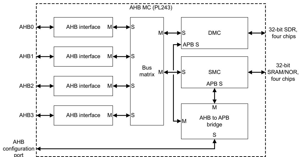
Figure 1-1 AHB MC (PL243) configuration
