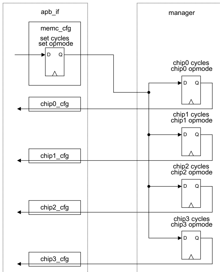
Figure 2-30 Chip configuration registers
