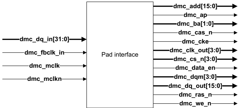
Figure 2-7 DMC pad interface external connections
