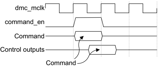
Figure 2-16 Command control output timing
