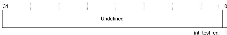
Figure 4-3 dmc_int_cfg Register bit assignments
