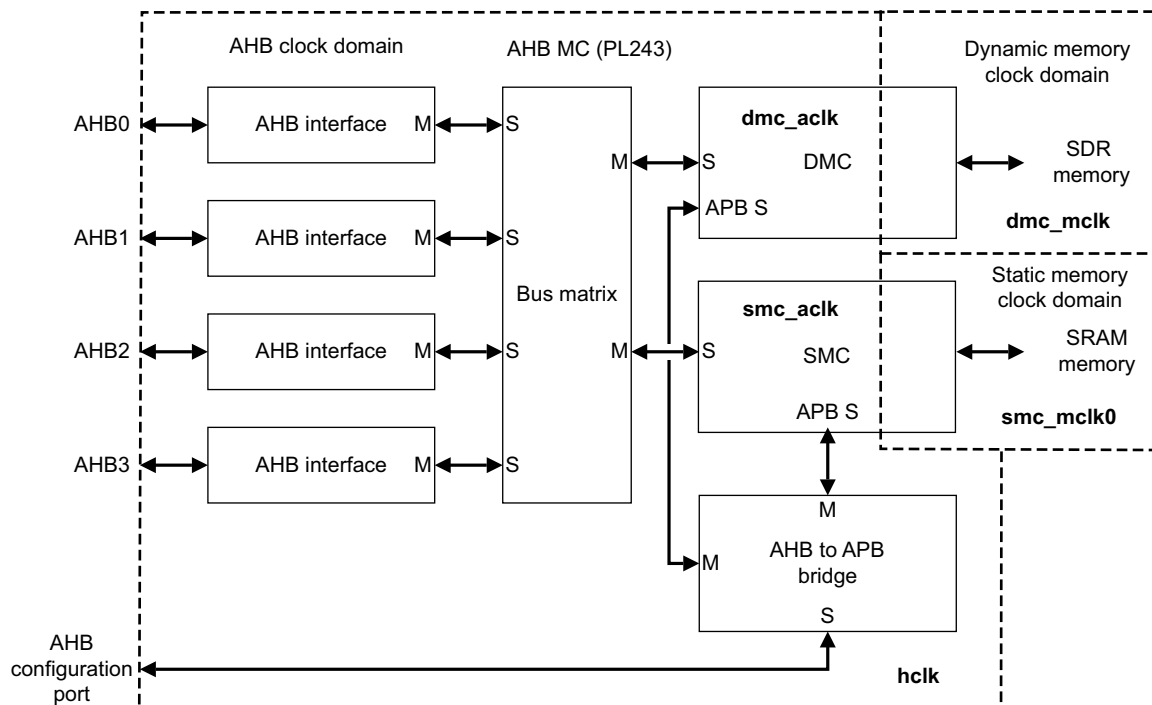
Figure 2-2 AHB MC (PL243) clock domains
