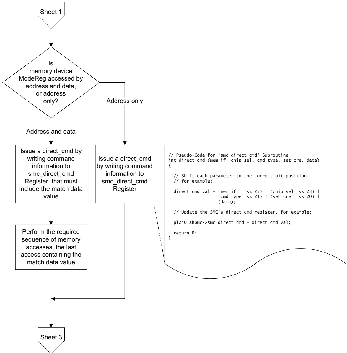
Figure 5-4 SMC and memory initialization sheet 2 of 3
