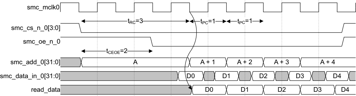
Figure 2-37 Page read
