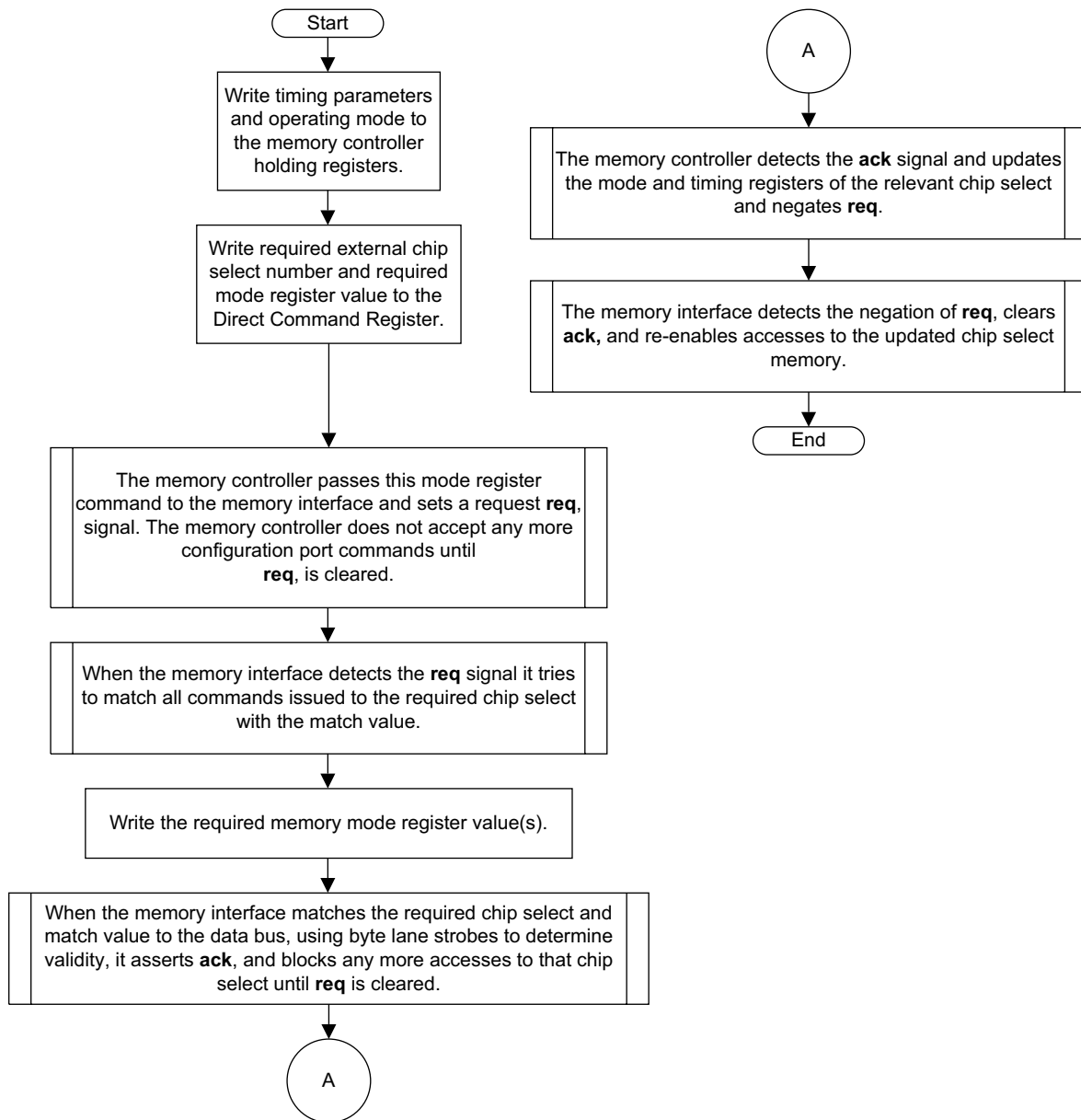
Figure 2-32 Software mechanism
