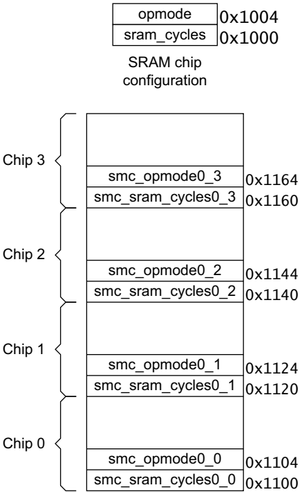
Figure 3-32 SMC chip configuration register map
