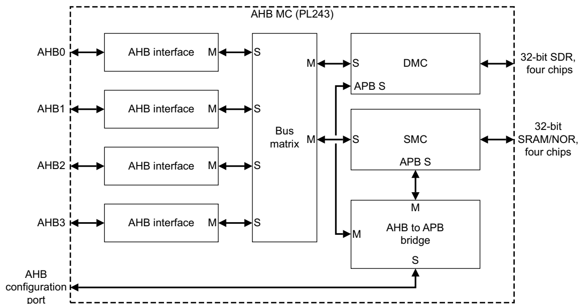
Figure 2-1 AHB MC (PL243) configuration
