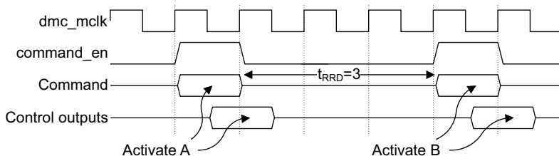
Figure 2-19 Bank activate to different bank activate for a memory timing, t_{RRD}
