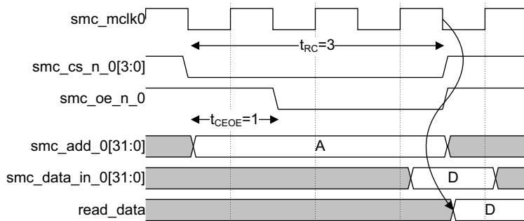
Figure 2-33 Asynchronous read
