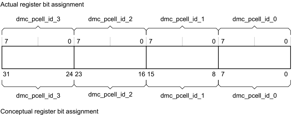
Figure 3-30 dmc_pcell_id Register bit assignments
