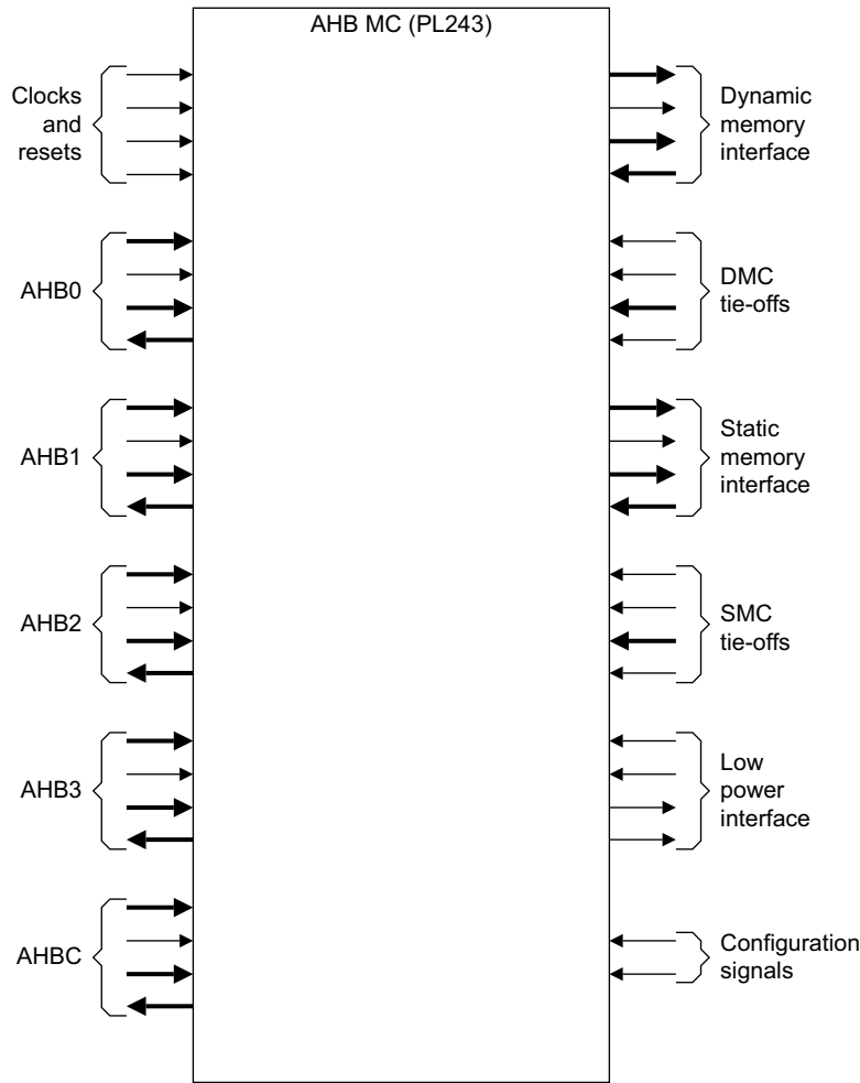
Figure A-1 AHB MC (PL243) grouping of signals
