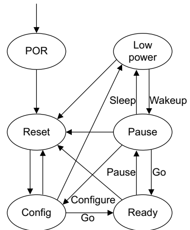
Figure 2-4 dmc_aclk domain FSM diagram
