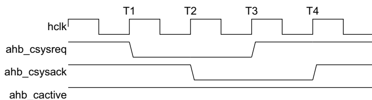
Figure 2-14 AHB domain denying a low-power request
