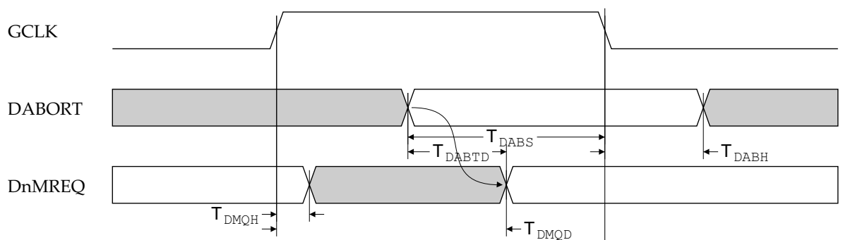
Figure 8-6 ARM9TDMI data ABORT and DnMREQ timing
