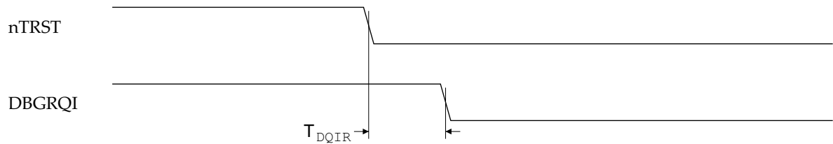
Figure 8-18 ARM9TDMI nTRST to DBGRQI relationship
