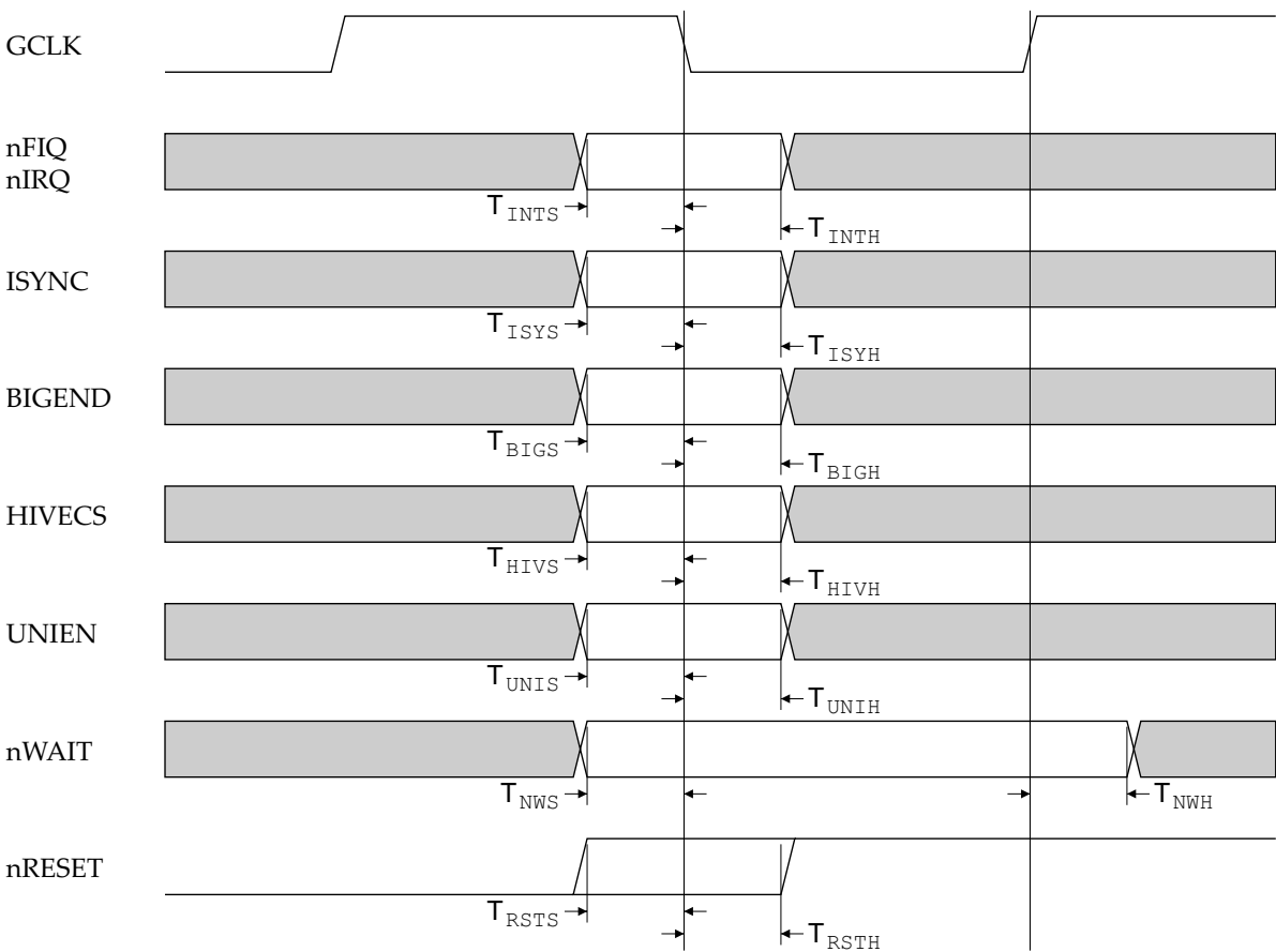
Figure 8-9 ARM9TDMI miscellaneous signal timing
