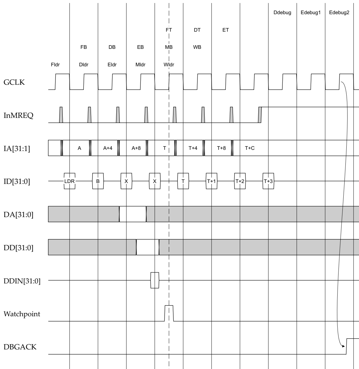
Figure 5-4 Watchpoint entry with branch
