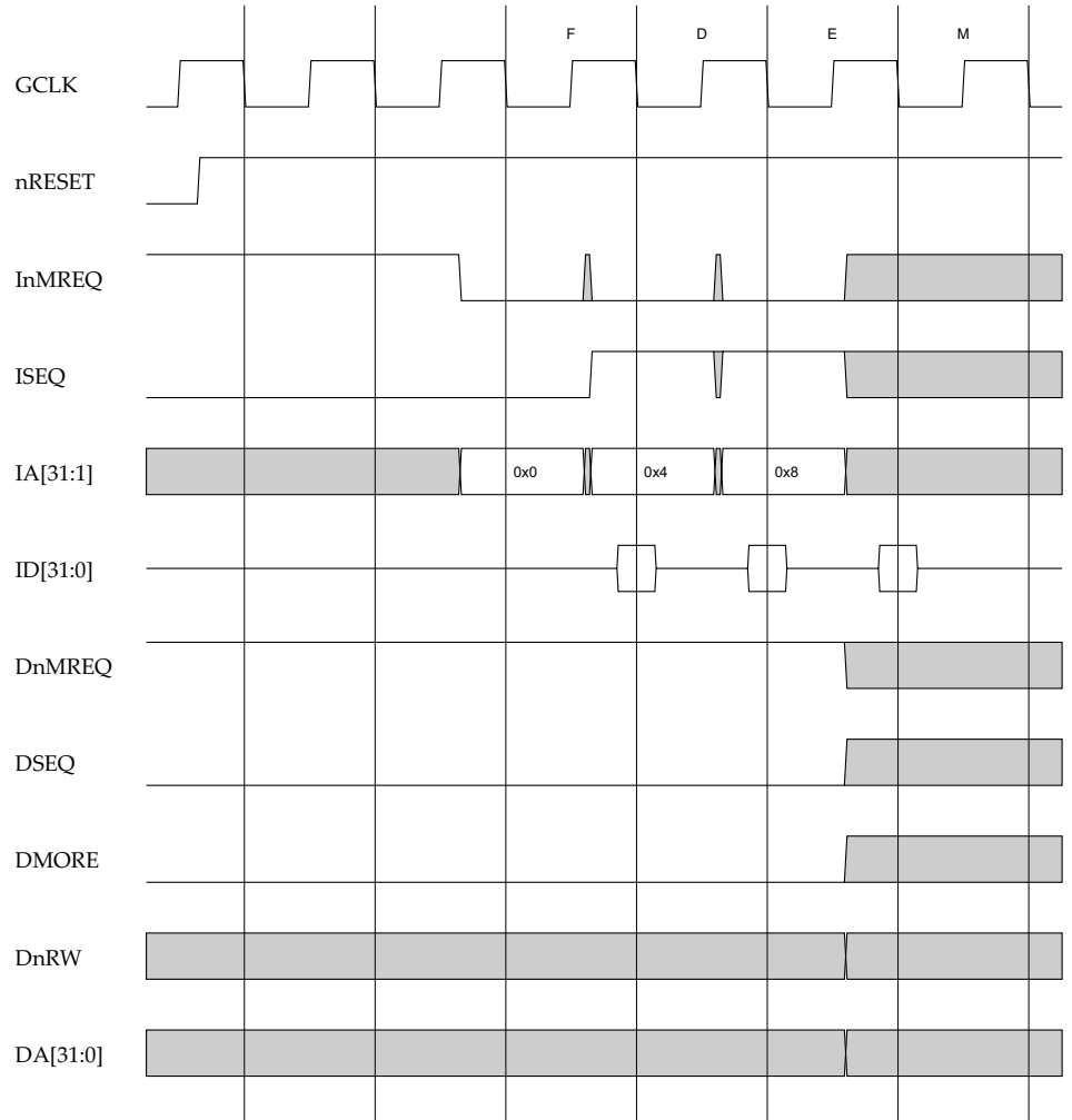
Figure 3-4 ARM9TDMI reset behavior
