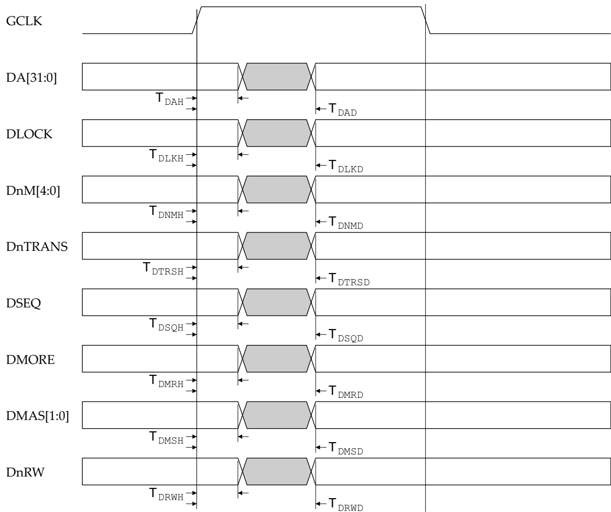
Figure 8-4 ARM9TDMI data memory interface output timing
