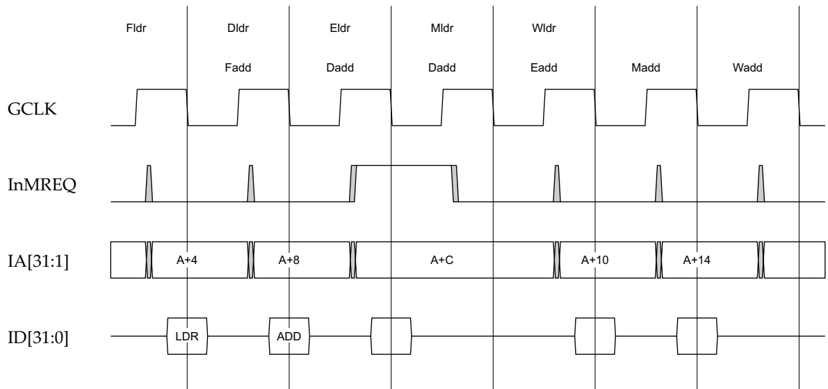
Figure 7-1 Single load interlock timing
