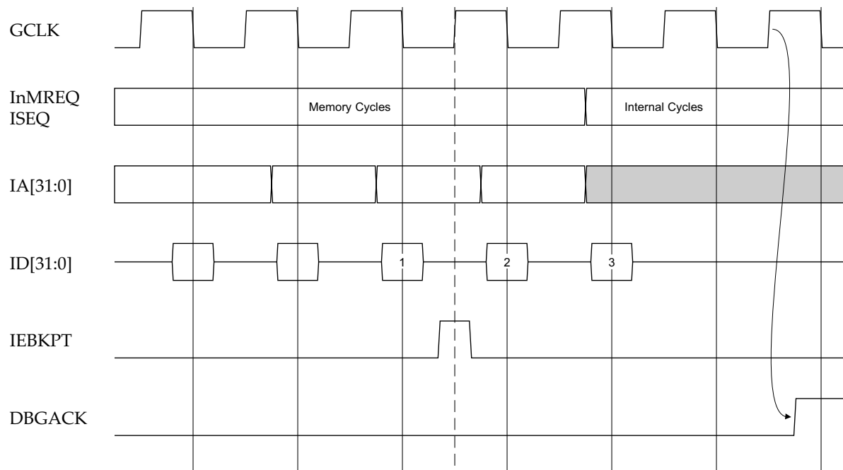
Figure 5-8 Debug state entry
