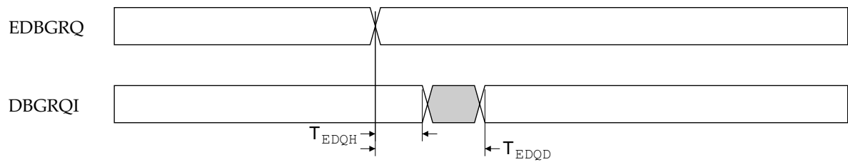
Figure 8-19 ARM9TDMI EDBGRQ to DBGRQI relationship
