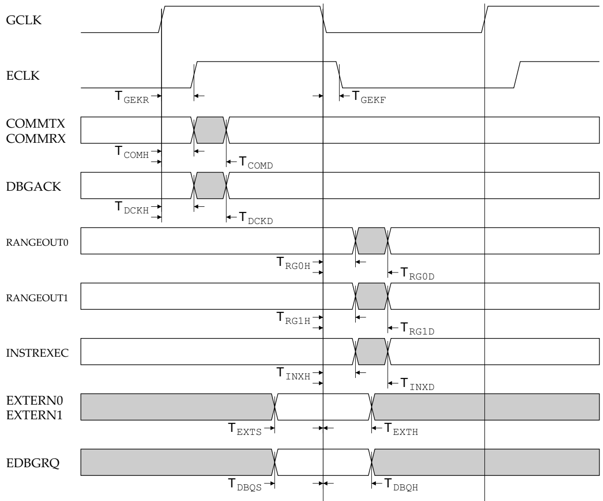
Figure 8-16 ARM9TDMI GCLK related debug output timings
