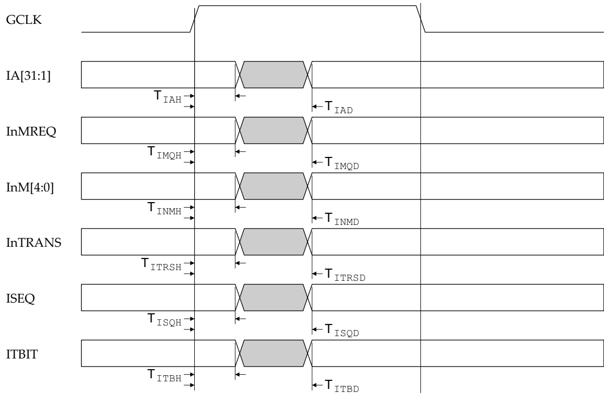
Figure 8-1 ARM9TDMI instruction memory interface output timing
