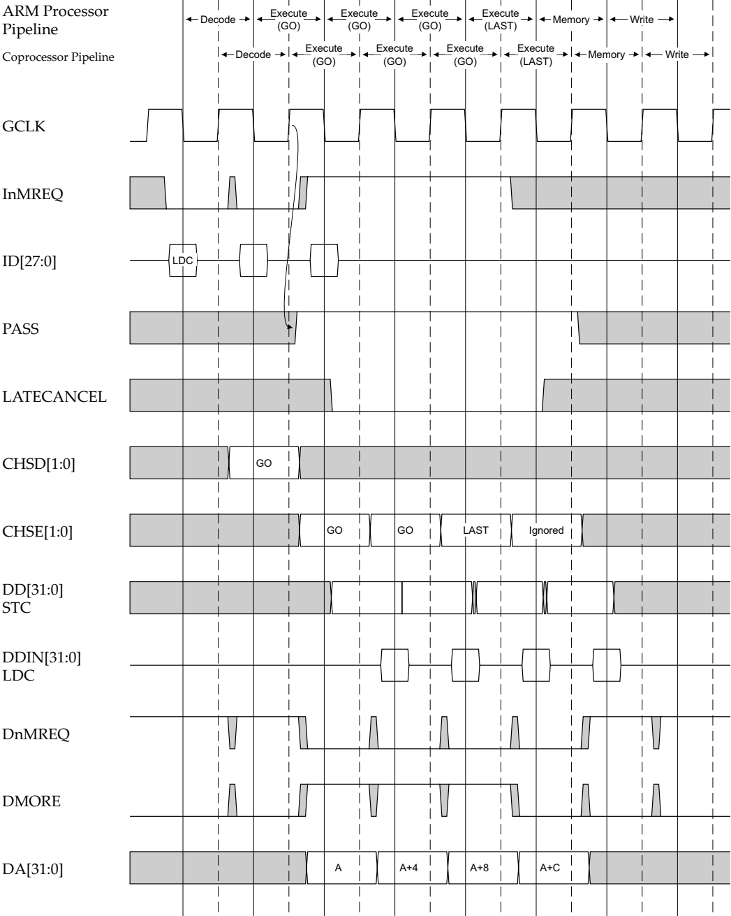
Figure 4-1 ARM9TDMI LDC / STC cycle timing
