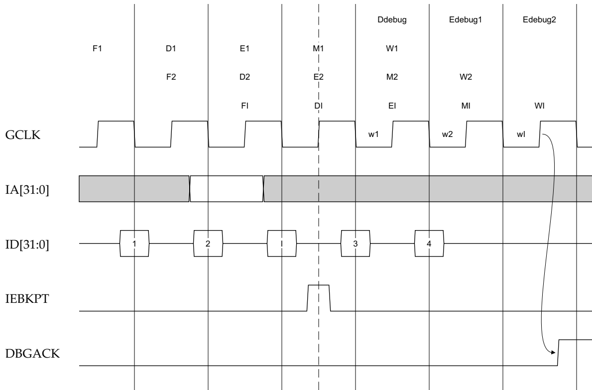
Figure 5-2 Breakpoint timing
