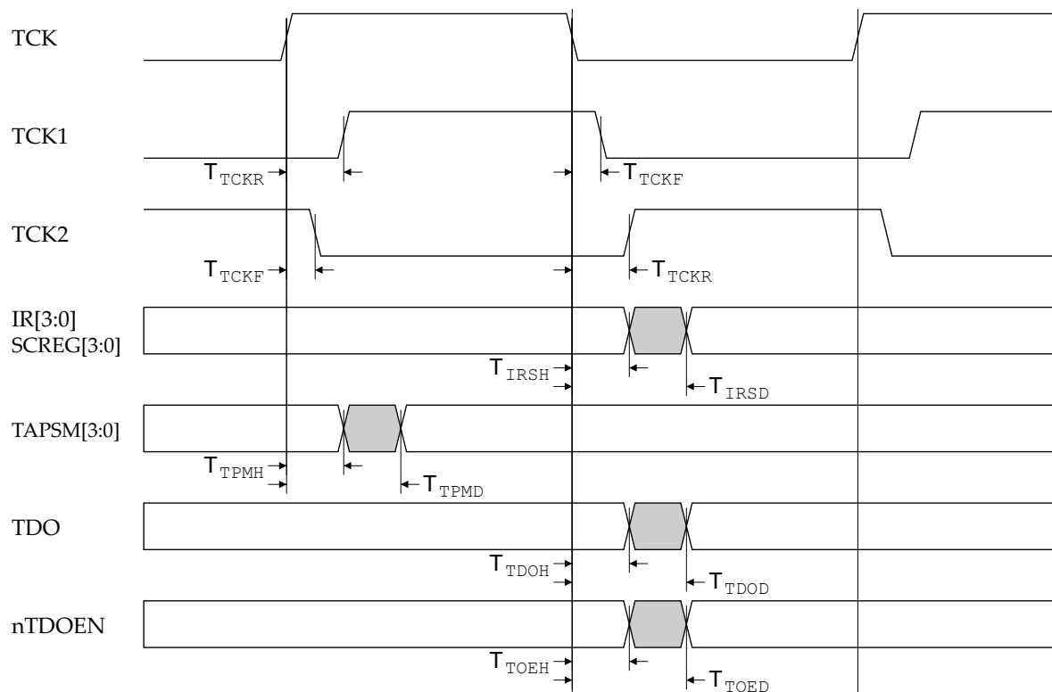
Figure 8-11 ARM9TDMI JTAG output signals
