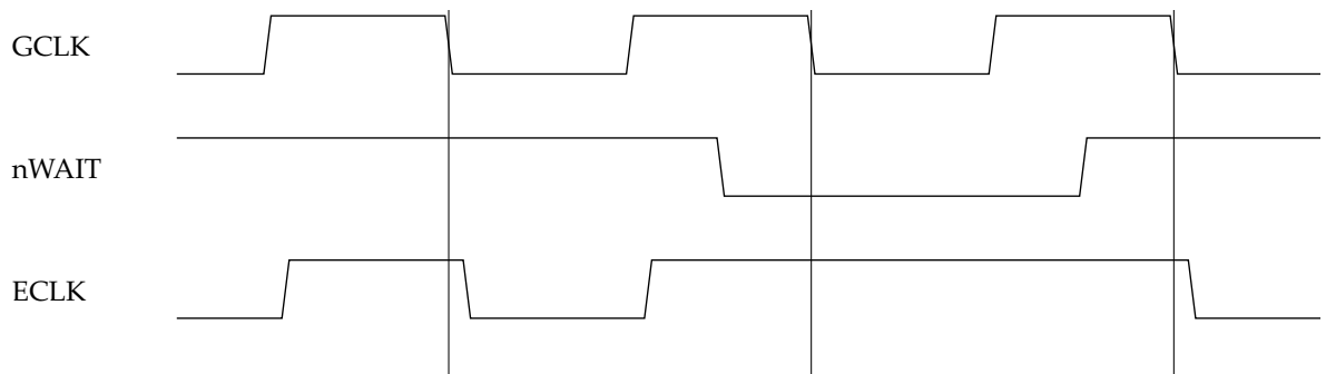
Figure 3-1 ARM9TDMI clock stalling using nWAIT
