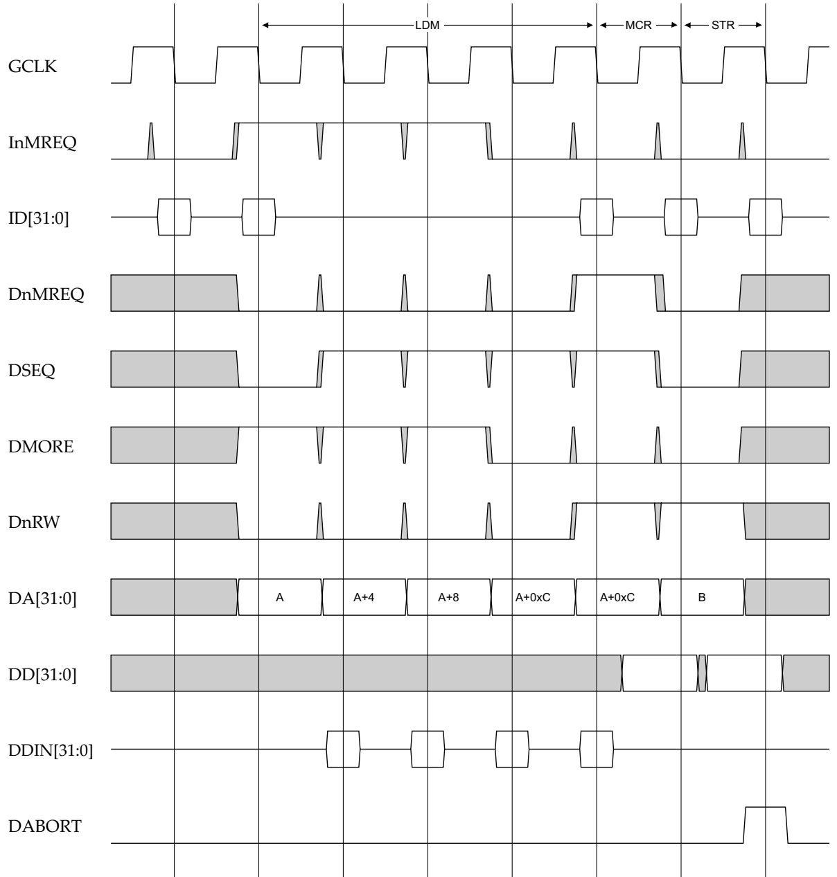
Figure 3-3 Data access timings
