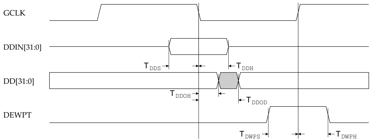
Figure 8-7 ARM9TDMI data data bus timing
