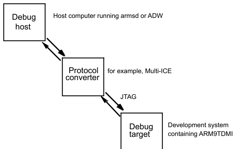
Figure 5-1 Typical debug system
