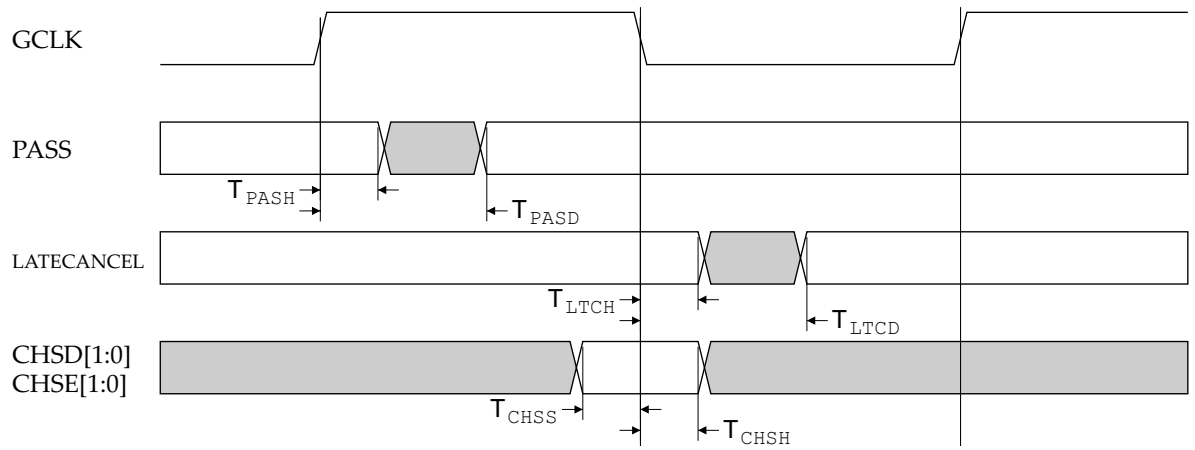
Figure 8-10 ARM9TDMI coprocessor interface signal timing
