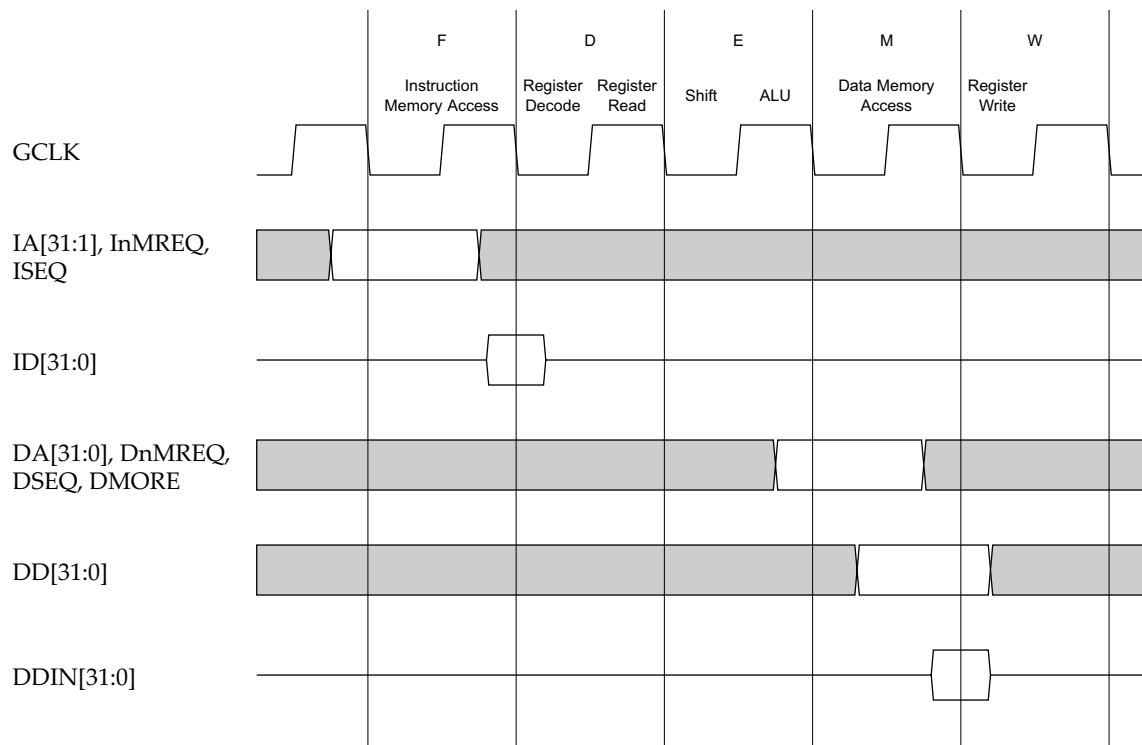
Figure 2-1 ARM9TDMI processor core instruction pipeline
