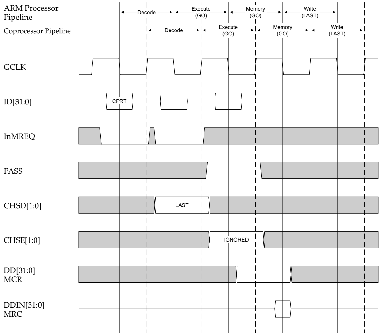
Figure 4-3 ARM9TDMI MCR / MRC transfer timing
