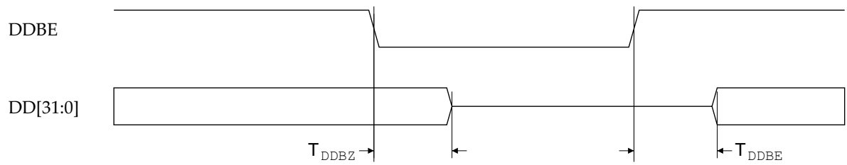
Figure 8-8 ARM9TDMI data bus enable
