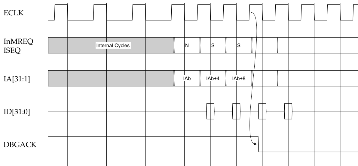
Figure 5-7 Debug exit sequence
