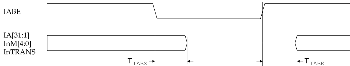
Figure 8-2 ARM9TDMI instruction address bus enable
