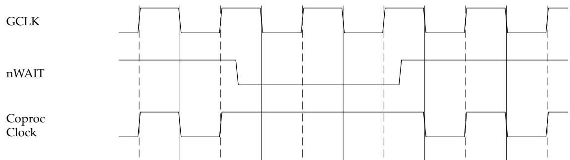
Figure 4-2 ARM9TDMI coprocessor clocking
