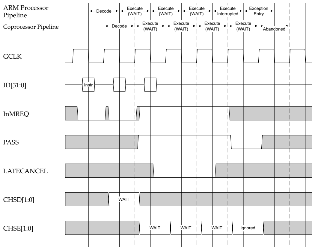
Figure 4-7 ARM9TDMI busy waiting and interrupts
