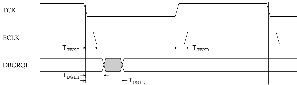
Figure 8-17 ARM9TDMI TCK related debug output timings
