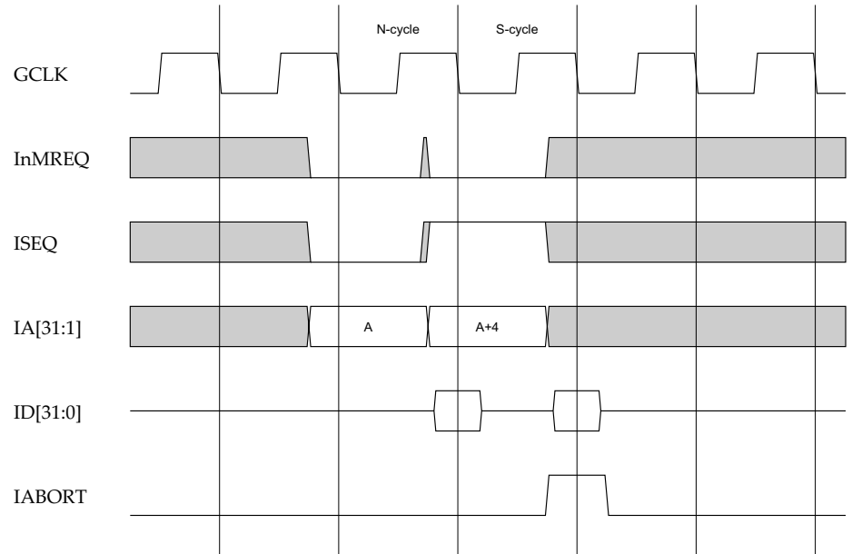
Figure 3-2 Instruction fetch timing
