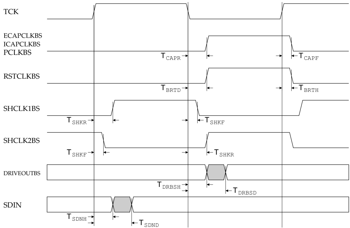
Figure 8-12 ARM9TDMI external boundary scan chain output signals
