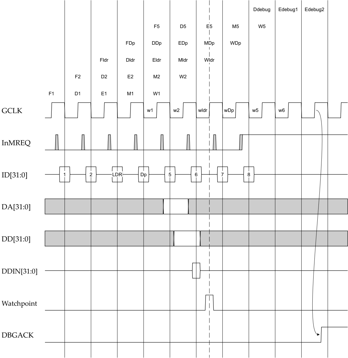
Figure 5-3 Watchpoint entry with data processing instruction
