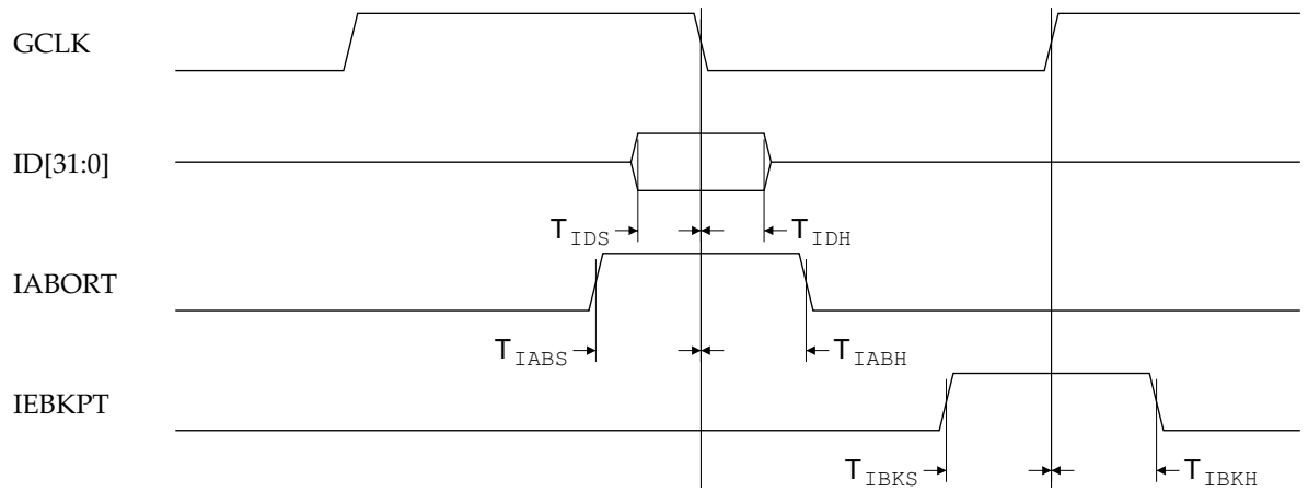
Figure 8-3 ARM9TDMI instruction memory interface input timing
