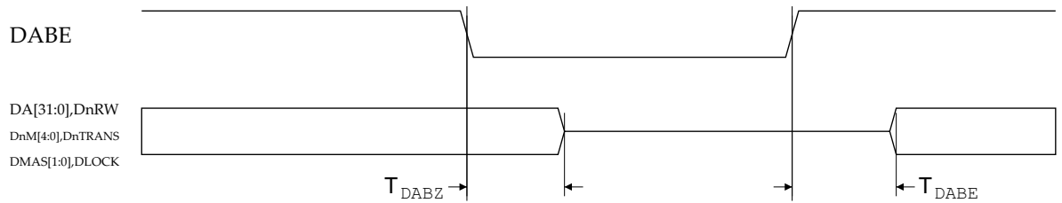
Figure 8-5 ARM9TDMI data address bus timing
