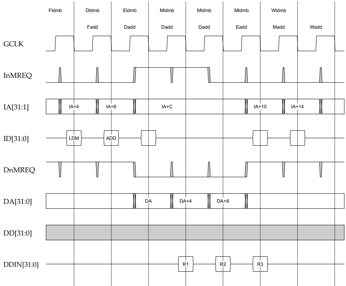
Figure 7-3 LDM interlock
