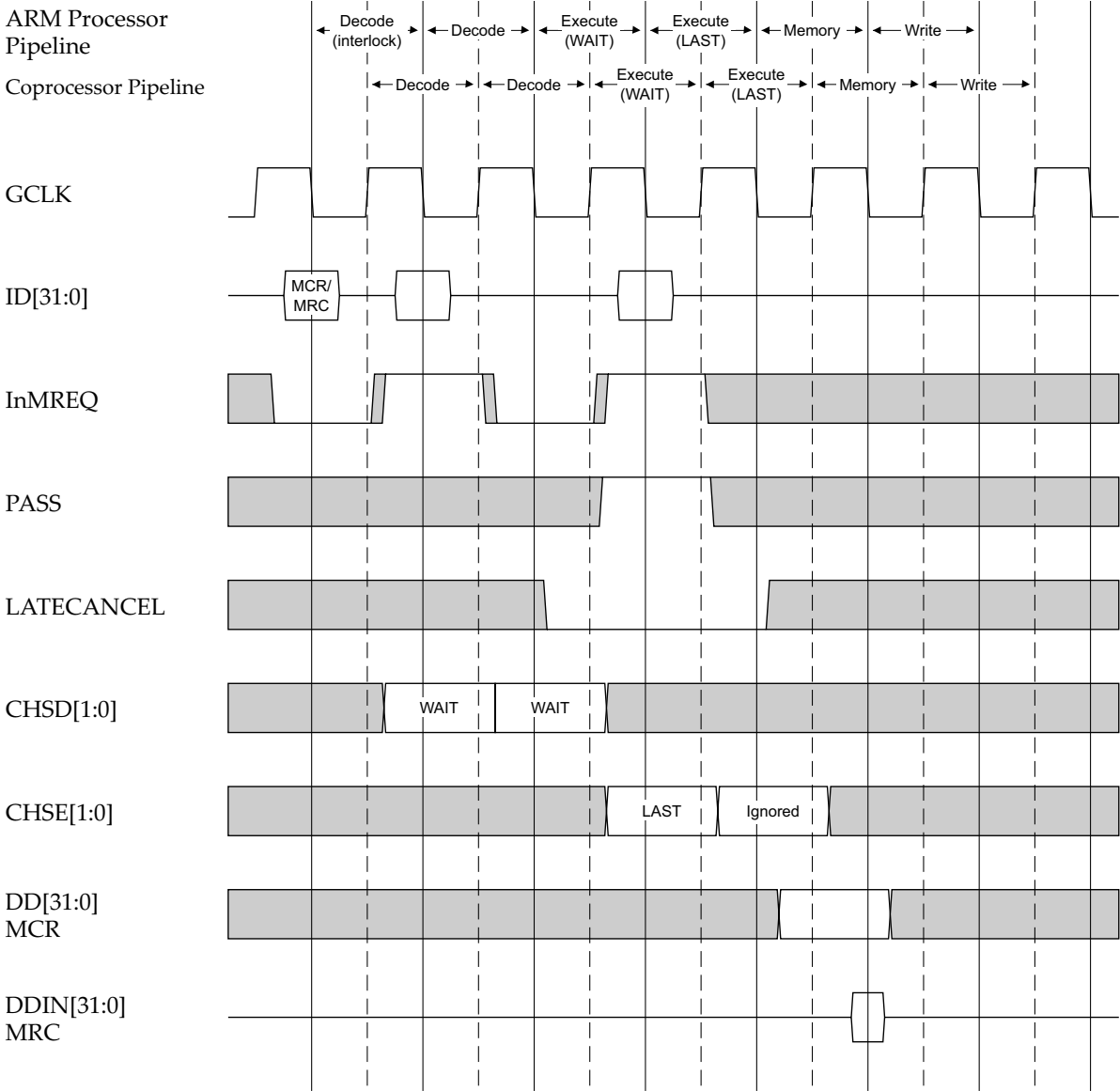
Figure 4-4 ARM9TDMI interlocked MCR
