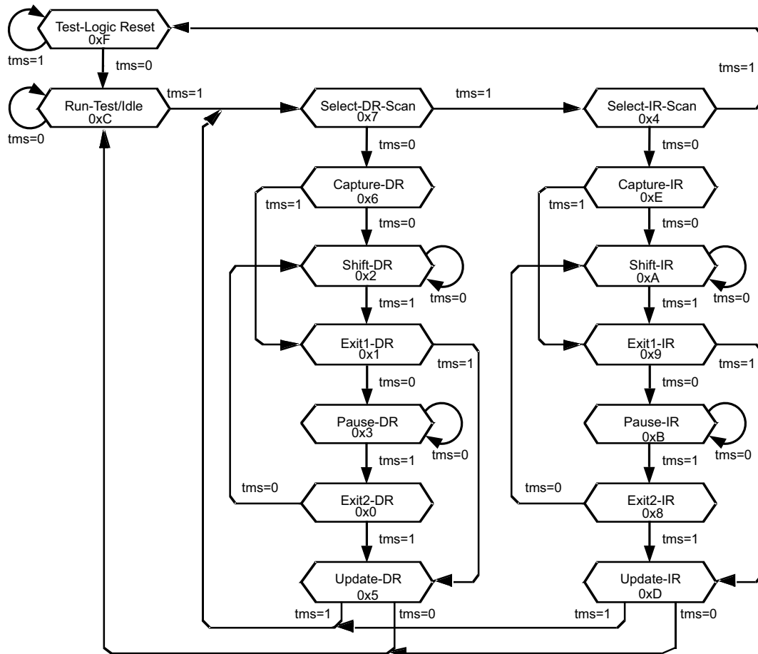
Figure 5-5 Test access port (TAP) controller state transitions
