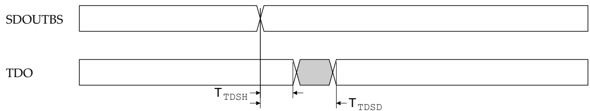
Figure 8-13 ARM9TDMI SDOUTBS to TDO relationship
