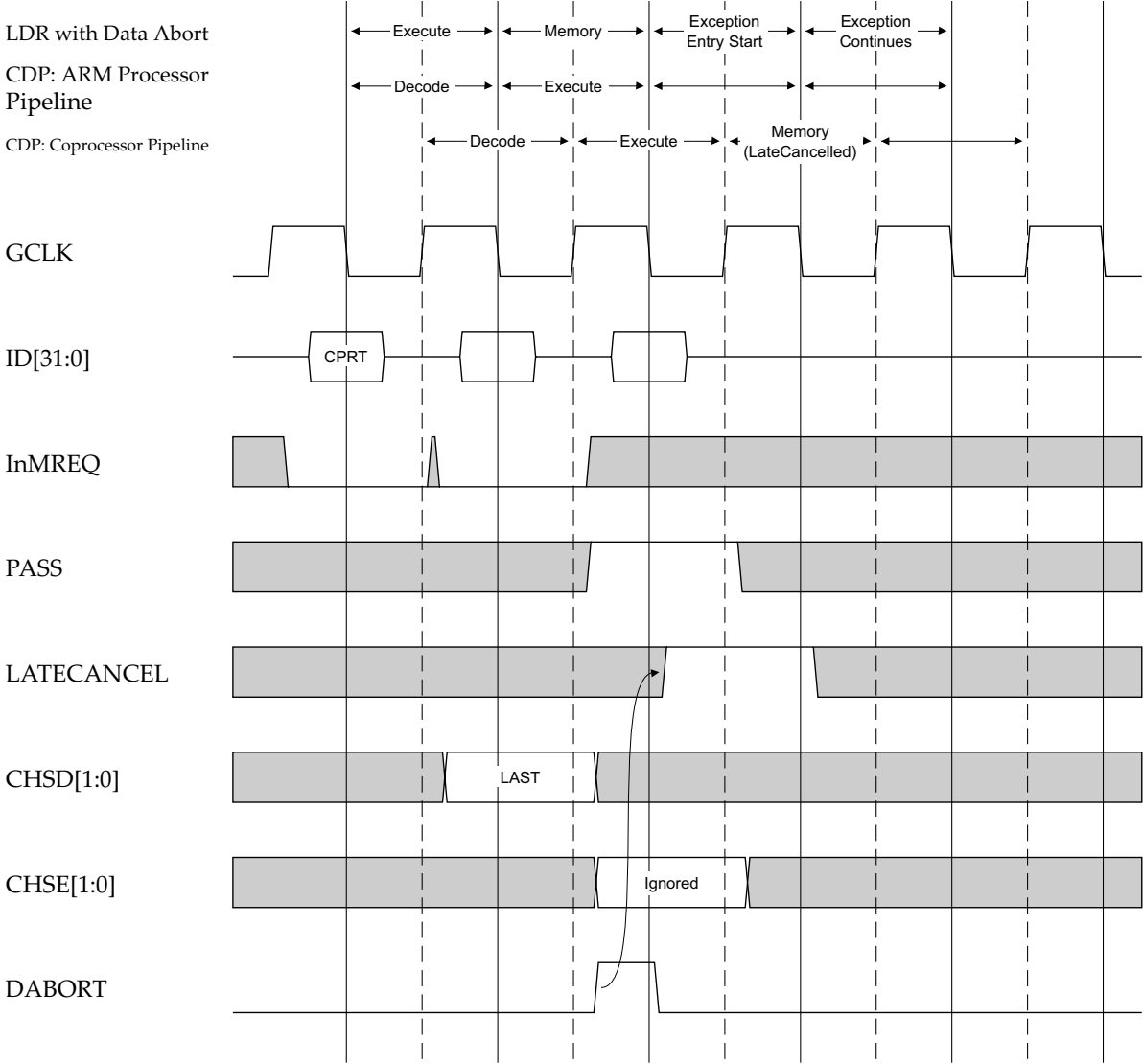
Figure 4-5 ARM9TDMI late cancelled CDP
