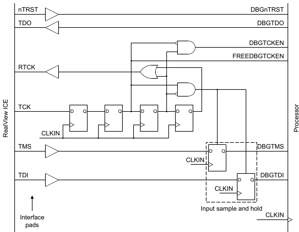
Figure 14-2 Clock synchronization
