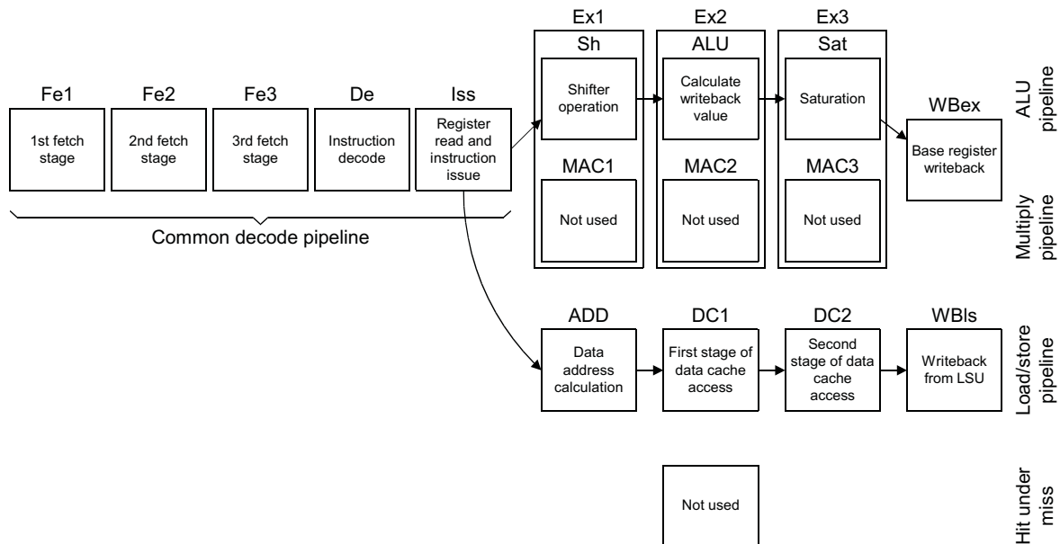
Figure 1-7 Progression of an LDR/STR operation
