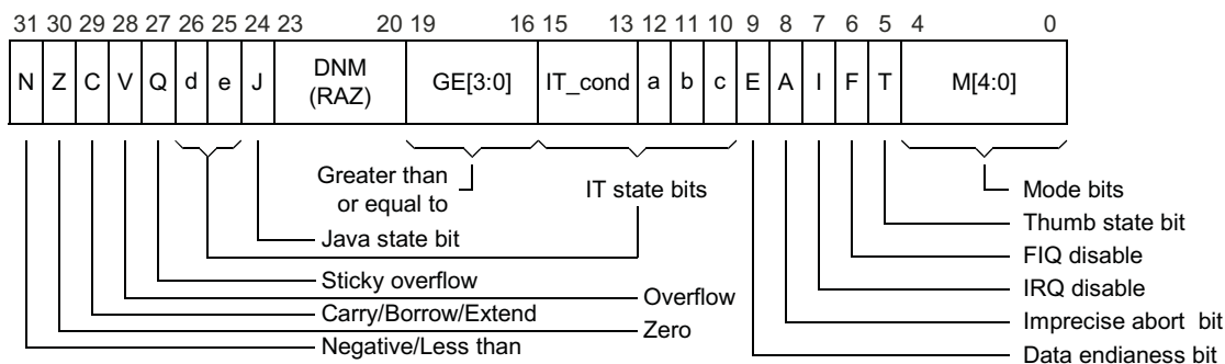
Figure 2-5 Program status register
