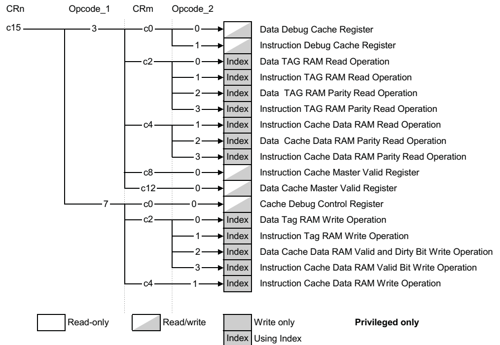
Figure 3-5 Cache debug and software test access registers
