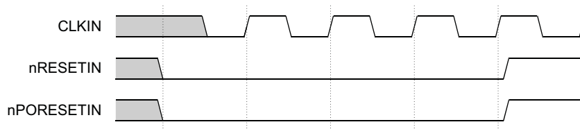
Figure 9-1 Power-on reset
