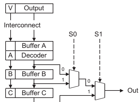
Figure 11-7 Instruction queue
