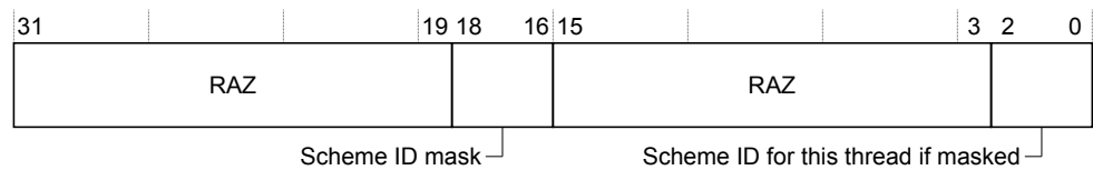
Figure B1-15 CLUSTERTHREADSIDOVR bit assignments
