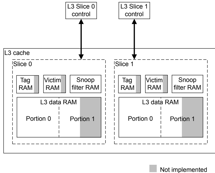
Figure A5-3 1.5MB or 3MB L3 cache implementation
