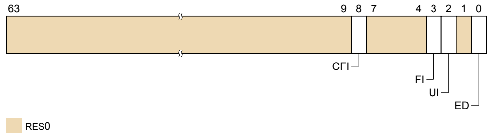
Figure B2-1 ERR1CTLR bit assignments
