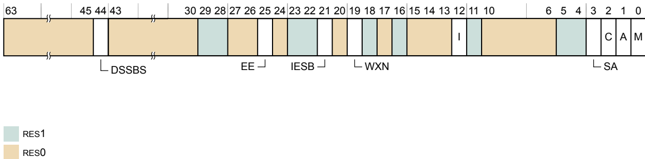
Figure B1-49 SCTL R _EL3 bit assignments
