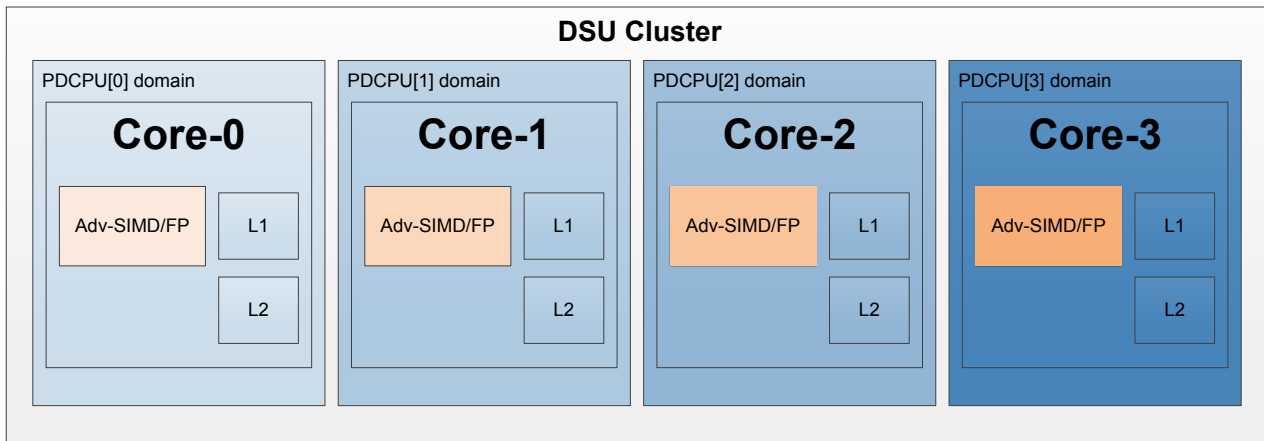
Figure A4-3 Cortex-A65 power domains
