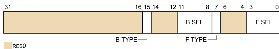
Figure D6-57 TRCSEQEVRn bit assignments
