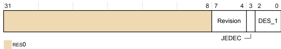
Figure D4-8 PMPIDR2 bit assignments
