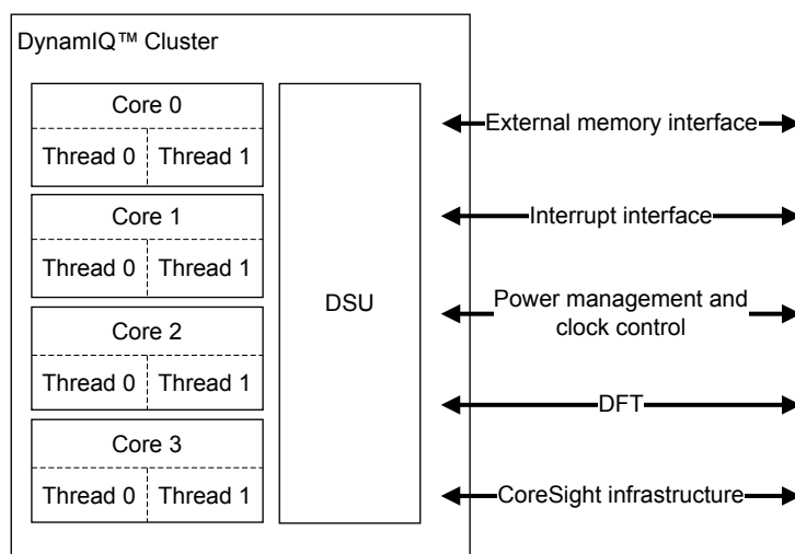
Figure A1-1 Example Cortex-A65 core configuration
