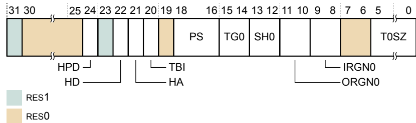
Figure B1-52 TCR_EL3 bit assignments
