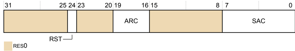
Figure D6-60 TRCSSCCR0 bit assignments
