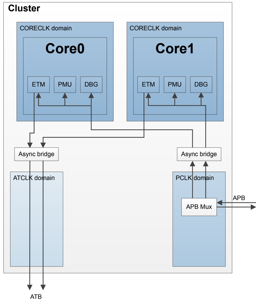
Figure C1-2 Cortex-A65 debug components
