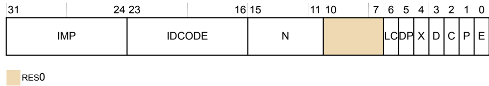
Figure D3-3 PMCR_EL0 bit assignments
