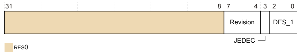
Figure D2-12 EDPIDR2 bit assignments
