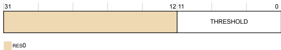
Figure D6-6 TRCCCCTL bit assignments
