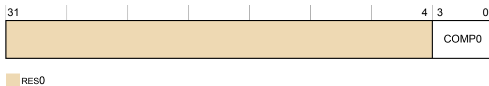
Figure D6-70 TRCVMIDCCTLR0 bit assignments
