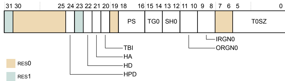
Figure B1-51 TCR_EL2 bit assignments
