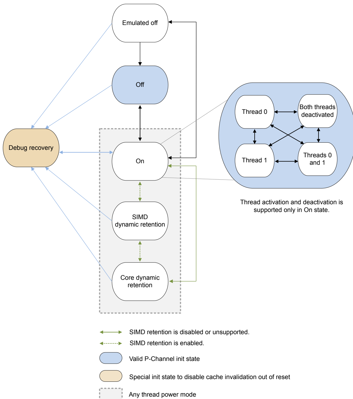
Figure A4-4 Cortex-A65 core power mode transitions
