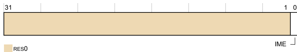
Figure D6-39 TRCITCTRL bit assignments
