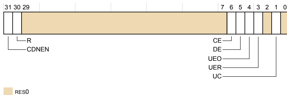
Figure B2-5 ERR0PFGCTL bit assignments
