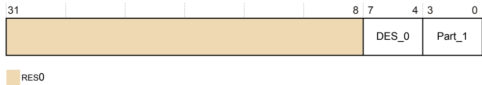
Figure D6-51 TRCPIDR1 bit assignments
