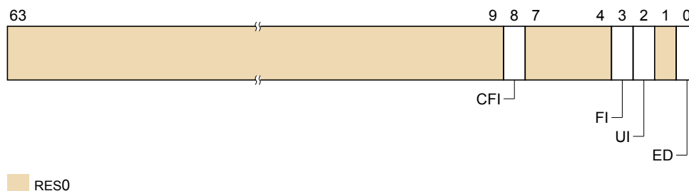
Figure B2-1 ERR0CTLR bit assignments
