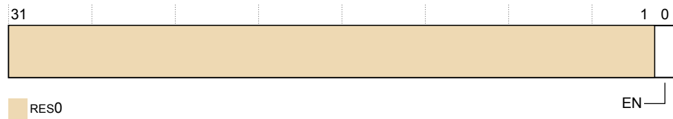
Figure D6-55 TRCPRGCTLR bit assignments
