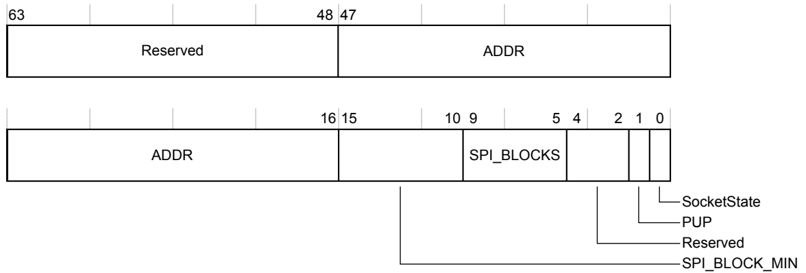
Figure 4-8 GICD_CHIPR<n> bit assignments
