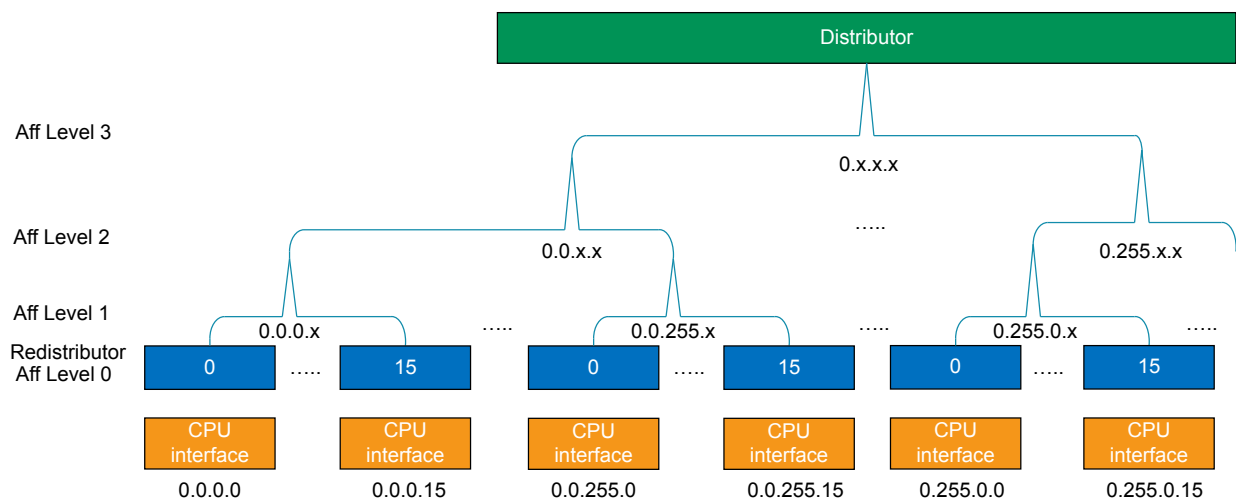
Figure 3-1 Affinity routing
