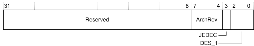
Figure 4-23 GICR_PIDR2 bit assignments
