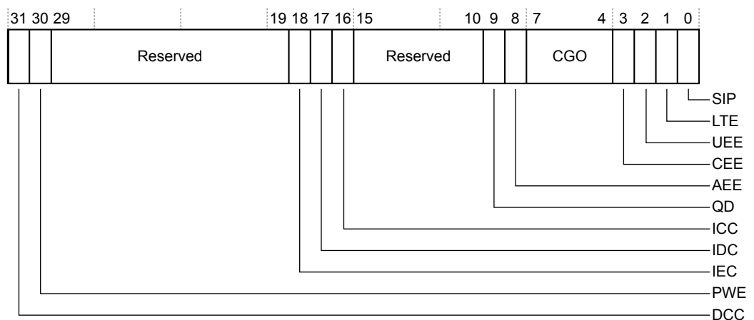
Figure 4-29 GITS_FCTLR bit assignments
