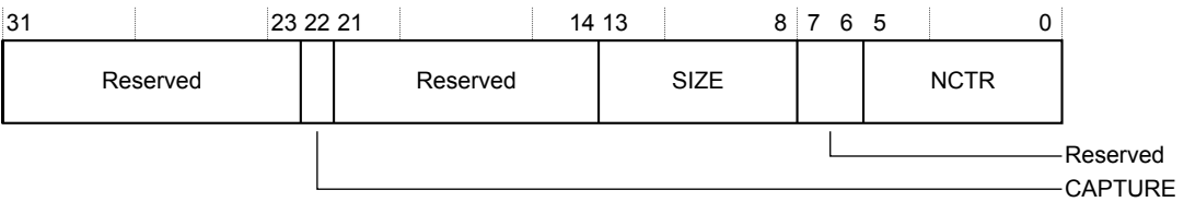
Figure 4-54 GICP_CFGR bit assignments
