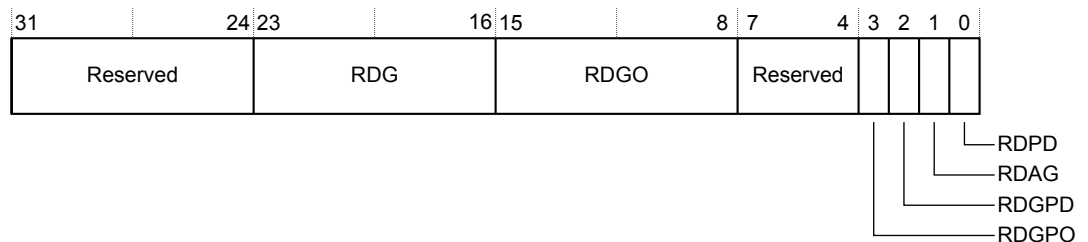
Figure 4-21 GICR_PWRR bit assignments
