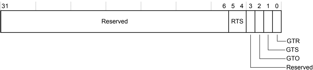
Figure 4-6 GICD_CHIPSR bit assignments
