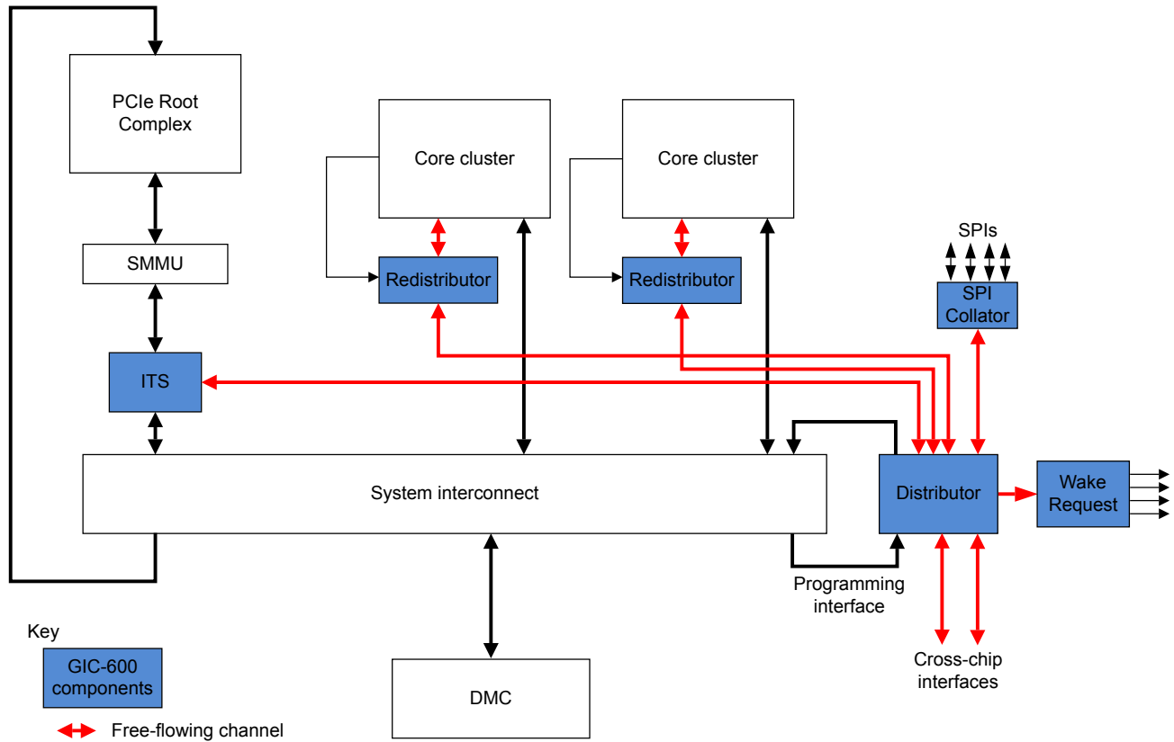
Figure 1-2 GIC-600 with interconnect in an example system
