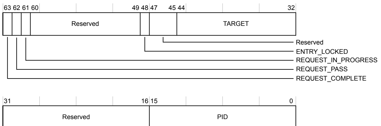
Figure 4-31 GITS_OPSR bit assignments
