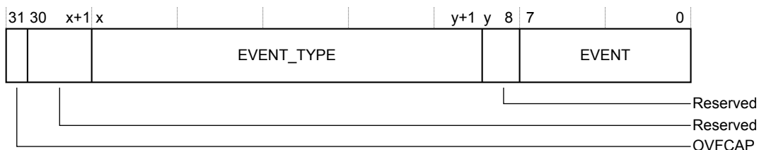
Figure 4-44 GICP_EVTYPERN bit assignments
