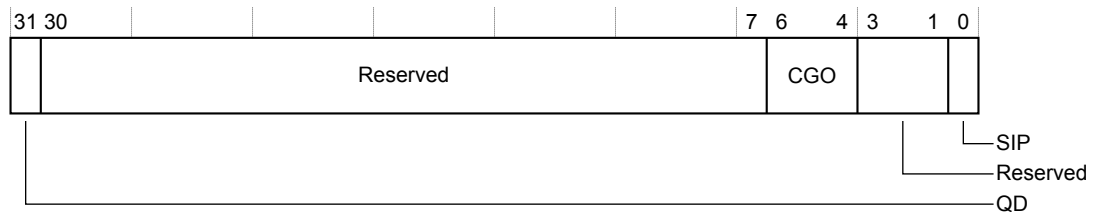
Figure 4-20 GICR_FCTLR bit assignments
